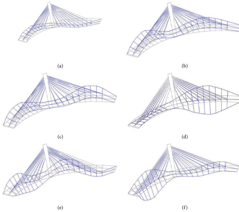
FIGURE 12: The representative experimental modes identified by the testing. (a) Mode 1 with f=0.635 Hz. (b) Mode 2 with f=0.996 Hz. (c) Mode 3 with f=1.143 Hz. (d) Mode 4 with f=1.387 Hz. (e) Mode 5 with f=1.523 Hz. (f) Mode 6 with f=1.602 Hz.
