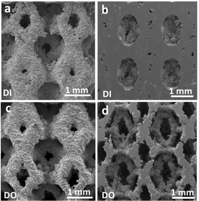
Fig. 4. SEM images of up skin surface (4a and 4c) and inner structure (4b and 4d) of DI and DO geometries.
