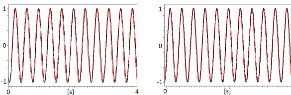
Fig. 12. Experiments of Subsection B. Estimated \sin(p\theta) (i.e., \widehat{\sin(p\theta)}_f ) for Observers I and II in [30], in comparison with the corresponding actual profiles.
