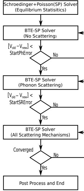
Fig. 1: Novel iteration scheme used to reduce the computational burden. By appropriately choosing the values of StartPhError and StartSRError we can reduce the simulation time significantly.
