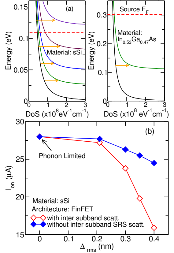
Fig. 7: (a) Plot of energy versus DoS for FinFET based on strained silicon and In_{0.53}Ga_{0.47}As . The lowest subband minima is taken as a reference in both the cases. (b) Plot of on-current versus surface roughness with and without intersubband surface roughness scattering.
