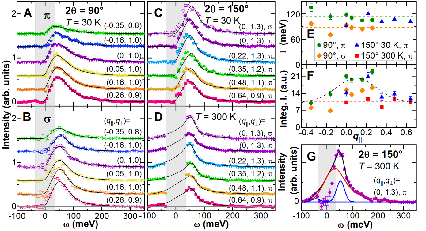
FIG. 2. A) and B) The q -dependence of the inelastic scattering of Zn-barlowite \text{Zn}_{0.56} collected at T = 30 K and scattering angle 2\theta = 90^\circ in both A) \pi and B) \sigma polarizations. C) and D) The q -dependence of the inelastic scattering of \text{Zn}_{0.56} collected at C) T = 30 K and D) T = 300 K at 2\theta = 150^\circ . Both \sigma (open symbols) and \pi (closed symbols) polarization are shown. In A)–B), the data were fit with a damped harmonic oscillator (DHO) curve from -100 – 500 meV with the DHO center fixed at 65 meV. In C)–D), the data were fit with a DHO and a phonon mode (see Supplemental Material, Section IE) from -100 – 500 meV, masking out -35 – 35 meV. The best fits are shown as black lines. The shading denotes in A)–B) a region of high uncertainty due to the elastic subtraction and in C)–D) these region were masked out during fitting. Vertical offsets were applied to separate the spectra. E)–F) The fitted DHO width \Gamma and integrated intensity as a function of q_{\parallel} . Horizontal dashed lines denote average values, while curves are guides to the eye. G) An example of the “DHO + phonon” model showing the fit components (red and blue lines, respectively) and the overall fit (black line).
