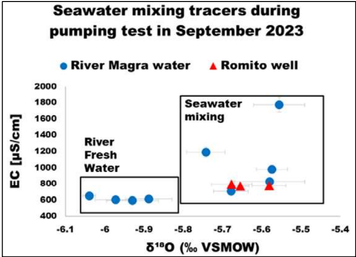
Figure 9 – Application of the EC- \delta^{18}\text{O} pair to identify SI in groundwater in the Romito well. The EC- \delta^{18}\text{O} values of the groundwater are compared with the values measured in the surface waters of the R. Magra in the same days and representing freshwater-saltwater mixing.
