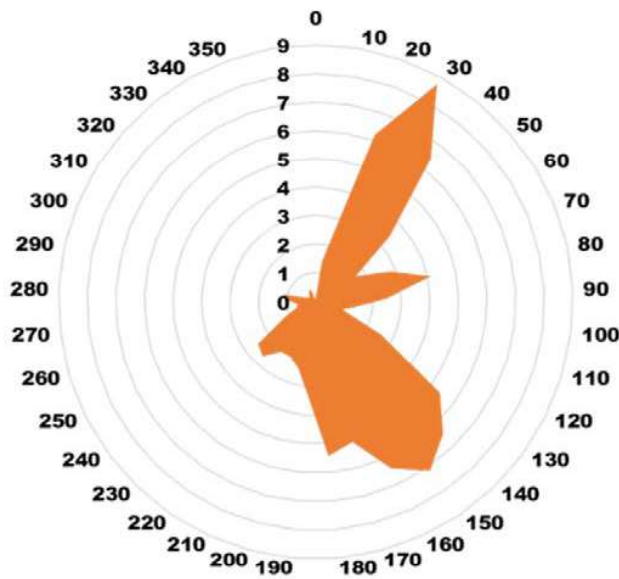
Figure 10 – Direction of dominant winds from 2010 to date in the study area (La Spezia tide gauge).
