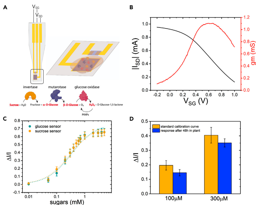
Figure 2. OEET-based sucrose and glucose sensors
