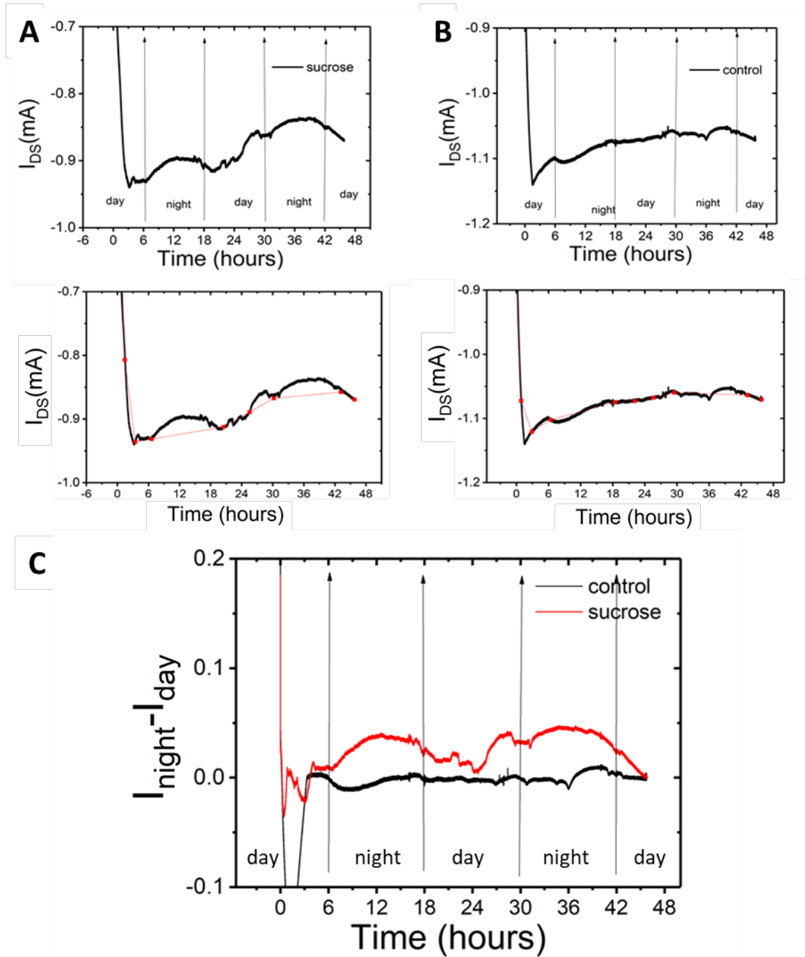
Figure S4: Baseline correction for in-vivo sensing measurements (Related to Figure 5). The drain current of sucrose sensor (A) and control device (B) was recorded for 48 hours in the xylem tissue. The baseline for both measurements was defined as the drain current values during day-time, I_{day} . (C) Corrected current temporal response ( I_{night} - I_{day} ) for 48 hours for sucrose sensor and control device.
