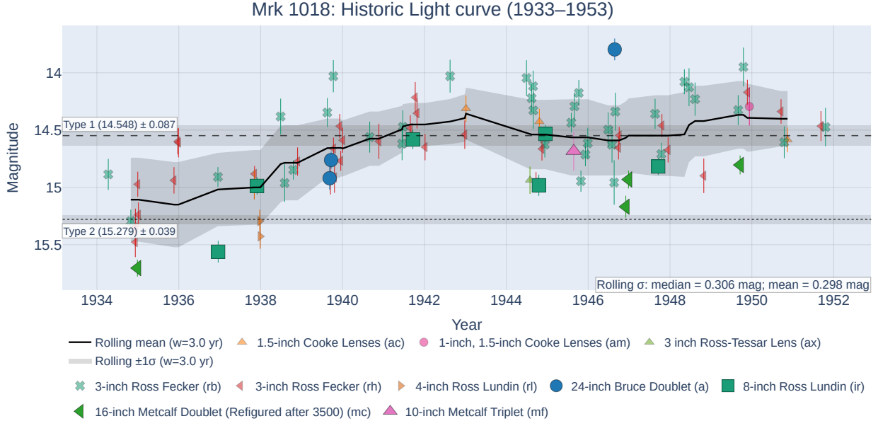
Figure 4. Mrk 1018's extreme event peaking around 1944. AGN + host flux contribution from historic DASCH Johnson B band magnitudes. The boxcar rolling mean (3 years width) is shown by the solid black line, with a 1\sigma grey band. Plates taken by telescopes larger than 8 inches have larger markers, whereas smaller telescopes are indicated with 55% opacity. Horizontal lines indicate Type 1 magnitude (SDSS; 2000–2010) and Type 2 magnitude (ASAS-SN; 2013–2018) with 1\sigma bands.
