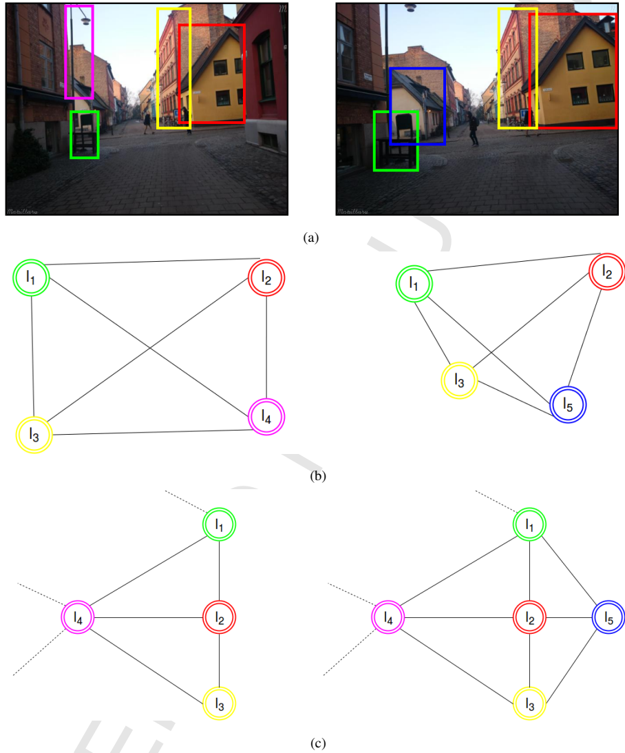
Figure 3: Incremental covisibility graph construction during the environment exploration. Examples of Edge Boxes landmarks extracted from images at time k - 1 (left) and at time k (right) respectively are shown in (3a). Relative landmark covisibility subgraphs of images visible at time k - 1 (left) and at time k (right) respectively are shown in (3b): landmarks acquired in the same image are connected in a dense graph. Landmark covisibility whole graph at time k - 1 (left) and at time k (right) respectively are shown in (3c): similar landmarks are mapped in the same node, while different landmarks produces new nodes.
