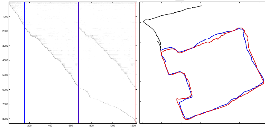
Figure 5: Trajectory and Clique matrix M_{clique} relative to the City Centre Dataset. This dataset presents a circular trajectory traversed two times starting from image 152 to image 674 and from image 675 to image 1220 and its clique matrix presents a repeating nodes pattern in the corresponding image indices, along with few new nodes that are specific of the second traversal. The allocation rate of new nodes is inferior in the second traversal with respect to the first traversal because the robot sees many landmarks belonging to already allocated nodes and only a small number of new nodes is allocated.
