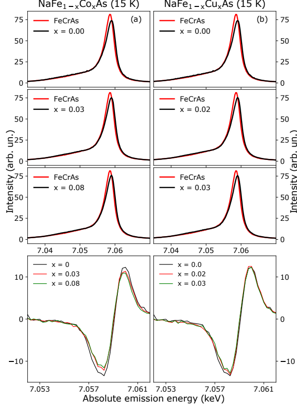
FIG. 3. (a) K_\beta XES for \text{NaFe}_{1-x}\text{Co}_x\text{As} with x = 0, 0.03 , and 0.08 at 15\text{ K} and spectrum of \text{FeCrAs} used as a reference for calculating the difference. (b) K_\beta XES for \text{NaFe}_{1-x}\text{Cu}_x\text{As} with x = 0, 0.02 , and 0.03 at 15\text{ K} and spectrum of \text{FeCrAs} used for calculating the difference. The last row is indicating the relative difference spectra for \text{NaFe}_{1-x}\text{Co}_x\text{As} and \text{NaFe}_{1-x}\text{Cu}_x\text{As} using as reference \text{FeCrAs} .
