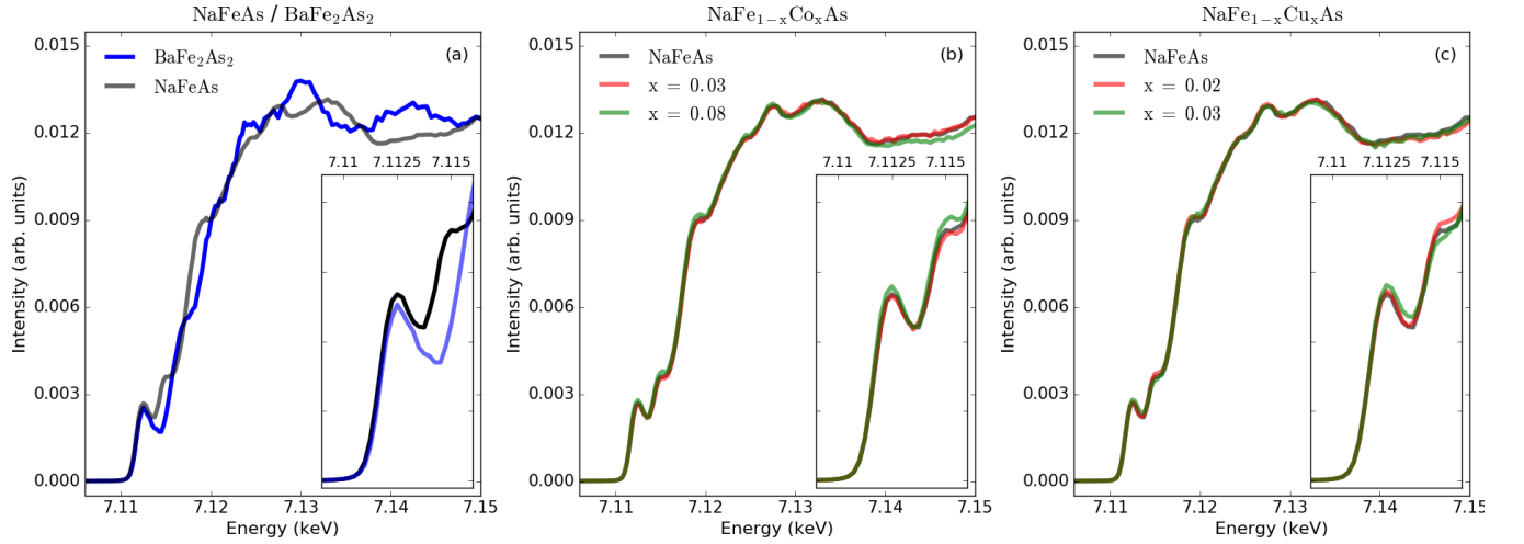
FIG. 2. (a) Fe-K edge XAS-PFY for BaFe 2 As 2 (blue solid line from Ref. 24 ) and NaFeAs (black solid line). Inset: Zoom on the pre-edge region for both compounds. (b) Fe-K edge XAS-PFY for NaFe 1-x Co x As for x=0 (black solid line), 0.03 (red solid line), and 0.08 (green solid line). Inset: Zoom on the pre-edge region for all the compounds. (c) Fe-K edge XAS-PFY for NaFe 1-x Cu x As for x=0 (black solid line), 0.02 (red solid line), and 0.03 (green solid line). Inset: Zoom on the pre-edge region for all the compounds.
