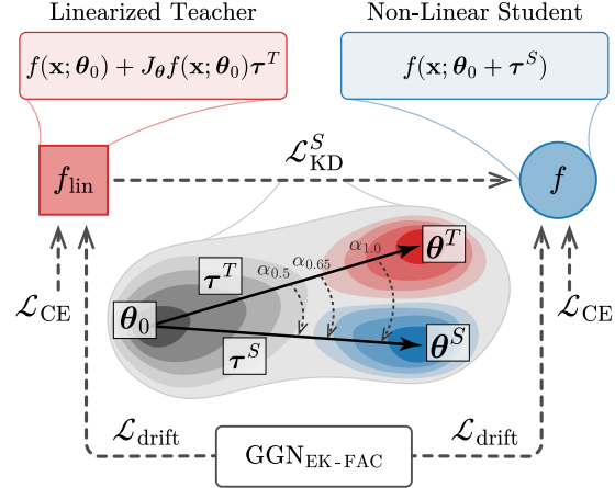
Figure 1. Overview. To improve weight disentanglement, a non-linear student model is fine-tuned by distilling a linearized teacher. Both models are trained with curvature-aware regularization based on an approximation of the Generalized Gauss-Newton matrix.
