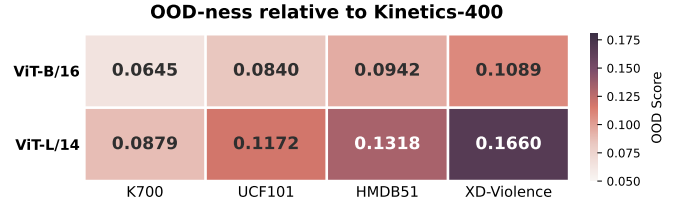
Fig. 3. For each dataset, we report its out-of-distribution (OOD) shift relative to K400, used to pre-train the base model. Larger values (e.g., for XD-Violence) indicate a stronger semantic mismatch with the source domain.
