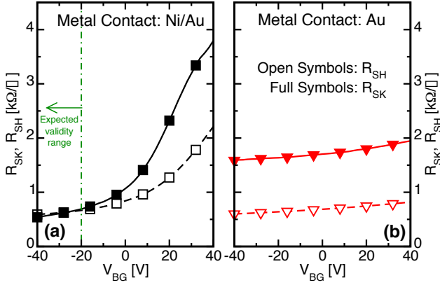
Fig. 9. Sheet resistance under the contact (full symbols) and in the channel (open symbols) for the Ni/Au stack (a) and the Au contact (b).
