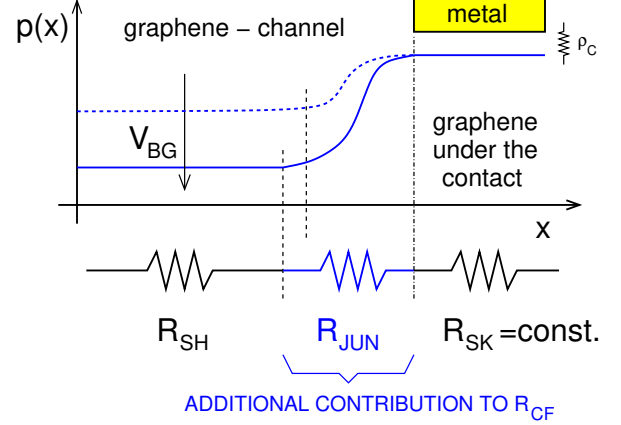
Fig. 10. Sketch of the hole density profile along the graphene in proximity of the contact edge. The step between the channel and the region under the contact (higher at large V_{BG} ) lead to a p - p^+ junction. The associated junction resistance R_{JUN} is not included in the transmission line model and it can impact the extracted graphene-metal contact parameters.
