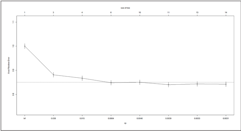
Graph 1. Variation of cross-validated error by cost of complexity.
