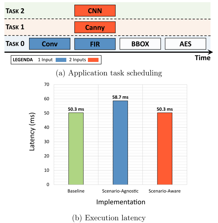
Fig. 9. Application task scheduling and execution latency concerning the three architectural variants of the overlay-based UAV companion computer.
