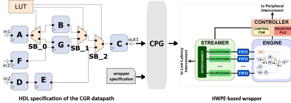
Fig. 5. MDC: From multi-dataflow specification to the generation of the HWPE wrapper.
