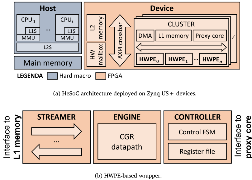
Fig. 3. Overview of the OOC components.
