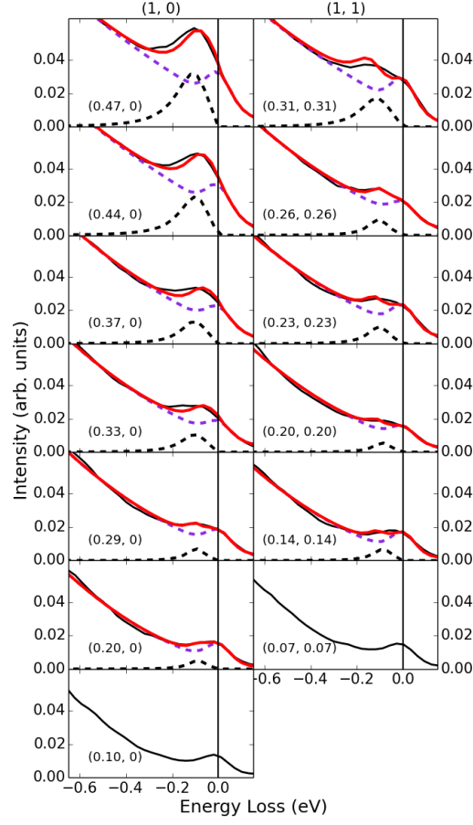
FIG. S1. Momentum dependence of RIXS spectra along (0, 0) \rightarrow (0.47, 0) and (0, 0) \rightarrow (0.31, 0.31 r.l.u.) for NaFeAs. Spectra were recorded in \pi polarization at the maximum of the Fe L_3 absorption edge at 10 K. Experimental data are shown as black solid line, fitting of background and elastic line are the purple dashed line and the magnetic peaks are depicted as black dashed line for every spectrum. The total fitting is depicted as red solid line. At low q_{\parallel} a fitting is unreliable, so no fitting is attempted.
