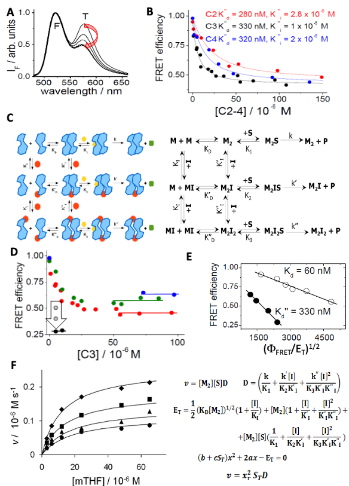
411 412 Figure 4. Spectroscopic and mechanistic analysis of hTS dissociative inhibition for 413 compounds C2, C3 and C4. A , Emission spectra of fluorescein(F)- and tetramethylrhodamine 414 (T)-labelled hTS ( \lambda_{\text{exc}} = 450 \text{ nm} ): the decreasing emission contribution of T relative to F with
