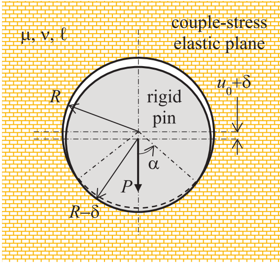
Fig. 1. Pin-hole contact configuration with clearance in a constrained couple-stress elastic medium.
