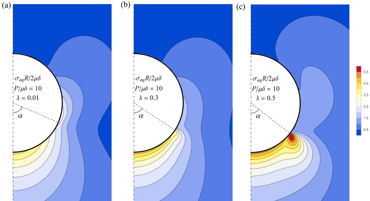
Fig. 6. Contour plots of the normalized von Mises equivalent stress, \sigma_{eq} R / (2\mu\delta) , in the vicinity of the hole under the curvature-compatible contact formulation. Results are shown for characteristic length \lambda = 0.01 (a), \lambda = 0.3 (b), and \lambda = 0.5 (c) at a fixed applied load P/(\mu\delta) = 10 .
