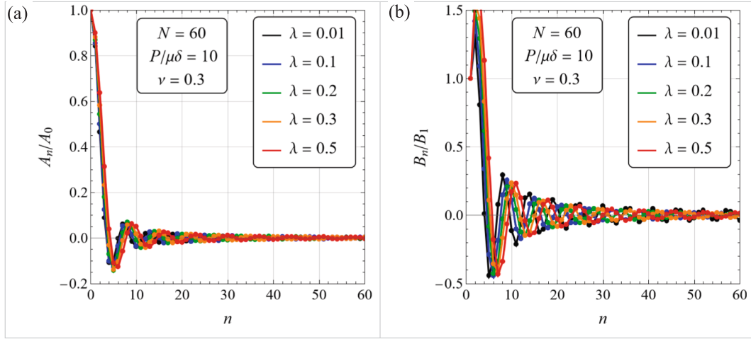
Fig. 7. Variations of the coefficient ratios A_n/A_0 (a), and B_n/B_1 (b), associated with the truncated system with N = 60 , shown for representative characteristic length ratios under constant applied pin load P = 10 \mu\delta .
