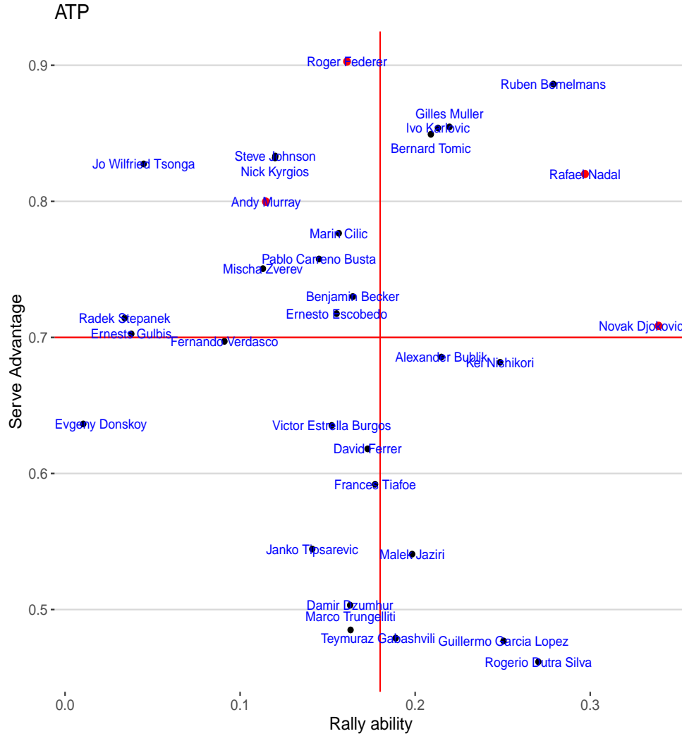
Figure 6: The posterior median rally ability \alpha_i estimated under the baseline model (Section 3.3), on the x -axis, against the total serve advantage (f_i(0) - f_i(15)) (Eq. (3)), on the y -axis, for male players in the ATP tournaments. The red lines represent the median rally ability of male athletes, parallel to the y -axis, and the median of the serve advantage. The red points indicate the top four players of the ATP tournaments. We only display those athletes whose 95% CI for serve advantage and rally ability do not include zero.
