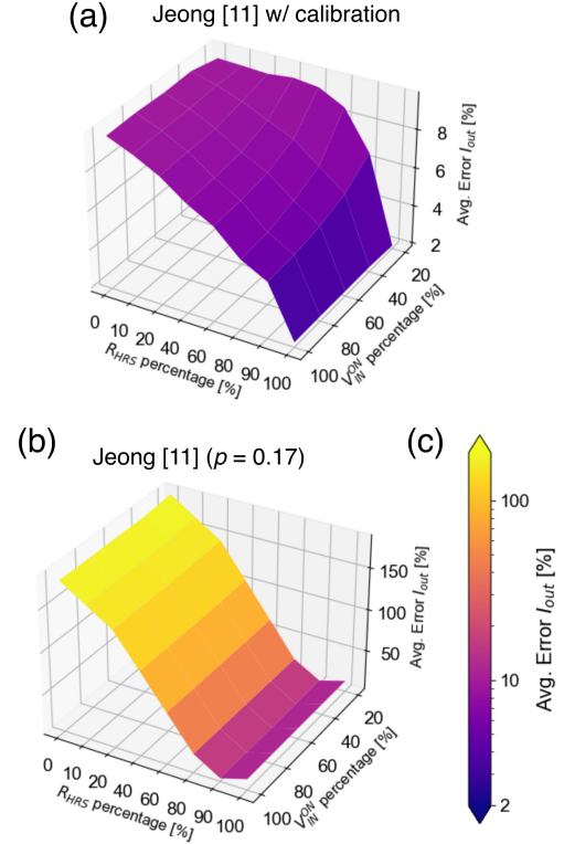
Fig. 6. Average output current estimation error for a 64 \times 64 crossbar array when (a) model in [11] with the proposed calibration procedure and (b) same model with the empirical p value from [11] are used. Each VMM typology is defined by the descriptors V_{in}^{\%} and R_{HRS}^{\%} . (c) reports the scale for the average error adopted in both plots.
