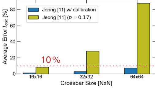
Fig. 7. Average output currents estimation error across 2000 VMMs for different crossbar sizes when using the model in [11] with and without the proposed calibration procedure.
