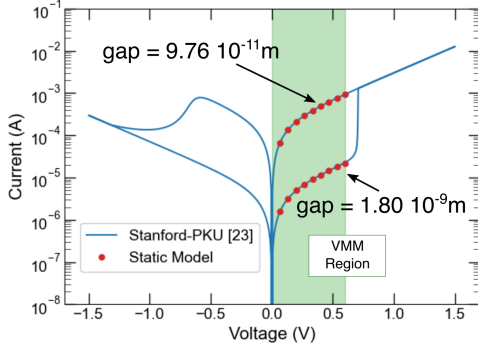
Fig. 10. I-V curve obtained with Stanford-PKU model fitted on IHP technology. The dotted lines represent the simplified modeling description restricted to the VMM operating region.
