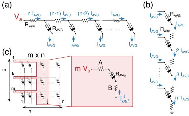
Fig. 2. Current redistribution along (a) input and (b) output metallization lines under assumptions in [11]. (c) Simplified circuit to compute correction factor for the resulting current on the j th output metal line based on [11].
