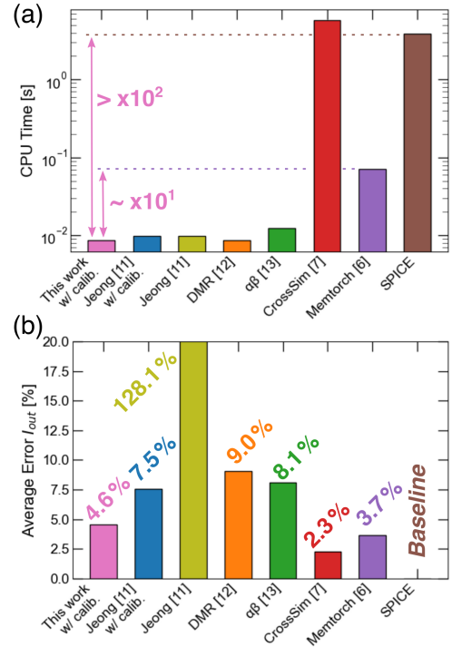
Fig. 13. (a) Average CPU time and (b) output current estimation error for 400 VMM operations on a 64 \times 64 array considering non-linear resistive devices.
