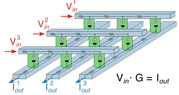
Fig. 1. 3 \times 3 crossbar structure performing a VMM operation in the electrical domain via resistive memory cells highlighted in green. We illustrate the parasitic wire resistances as lumped components.
