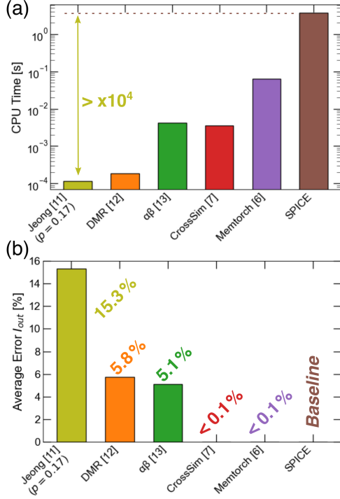
Fig. 3. (a) Average CPU time and (b) output current estimation error for 400 VMM operations on a 64 \times 64 array considering linear cross-points elements.
