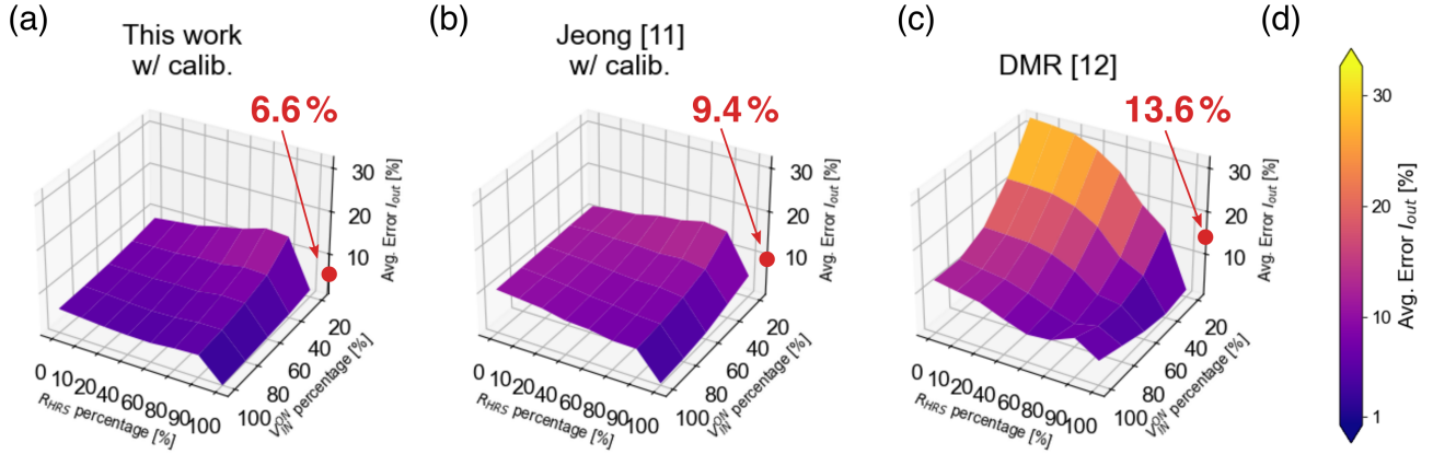
Fig. 14. Average output currents error estimation for random VMMs of different typologies ( V_{in}^{\%} , R_{HRS}^{\%} ) with (a) the proposed model with calibration, (b) model in [11] with calibration, and (c) DMR model. The red dot indicates the mean error across all VMM typologies. (d) Reports the scale for the average error adopted in all plots.
