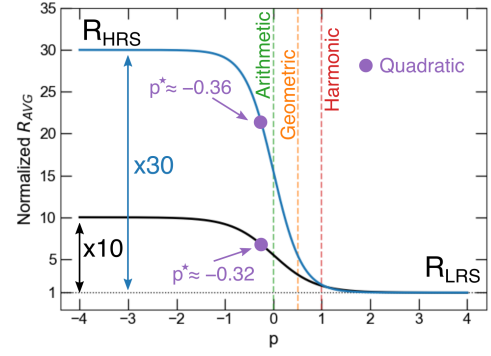
Fig. 4. Normalized resistance R_{AVG} as a function of p , shown for two memory windows ( R_{HRS}/R_{LRS} = 10 , black line, and 30 , blue line). We highlight the Pythagorean means.
