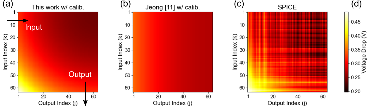
Fig. 12. Estimated voltage drop across each memory cell for a 64 \times 64 VMM operation with (a) proposed model with calibration, (b) model in [11] with calibration, and (c) nodal analysis in SPICE. (d) Reports the scale for the voltage drop adopted in all plots.
