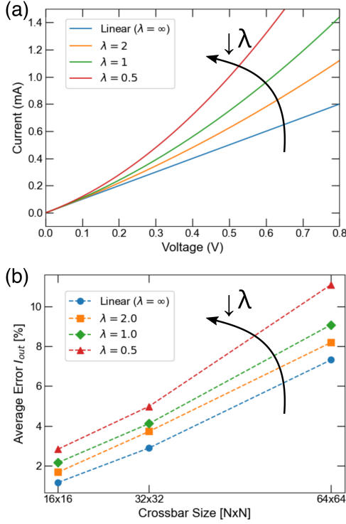
Fig. 9. (a) I-V characteristics for various \lambda values. (b) Average output currents estimation error by the model in [11] under different array sizes when the resistive memory cells' non-linearity is changed.
