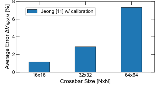
Fig. 8. Average voltage drop estimation errors across 50 VMM operations for various crossbar sizes using the model in [11] with the proposed calibration procedure. We bias input lines at 0.5 V and sample the weight matrices from a uniform distribution.
