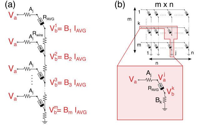
Fig. 11. (a) Proposed nodes level voltage drop modeling for a generic j th output line. (b) Equivalent circuit for an arbitrary (j, k) memory cell including the resistive parasitic elements.
