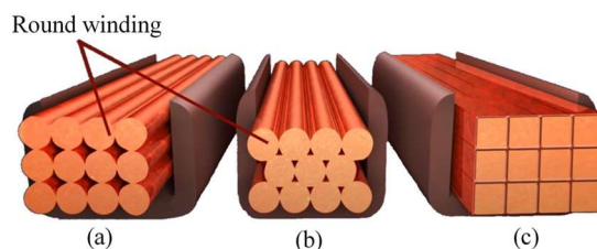
Figure 1 Qualitative view of a slot cross section for (a) regular round winding, (b) modified round winding, (c) rectangular winding
