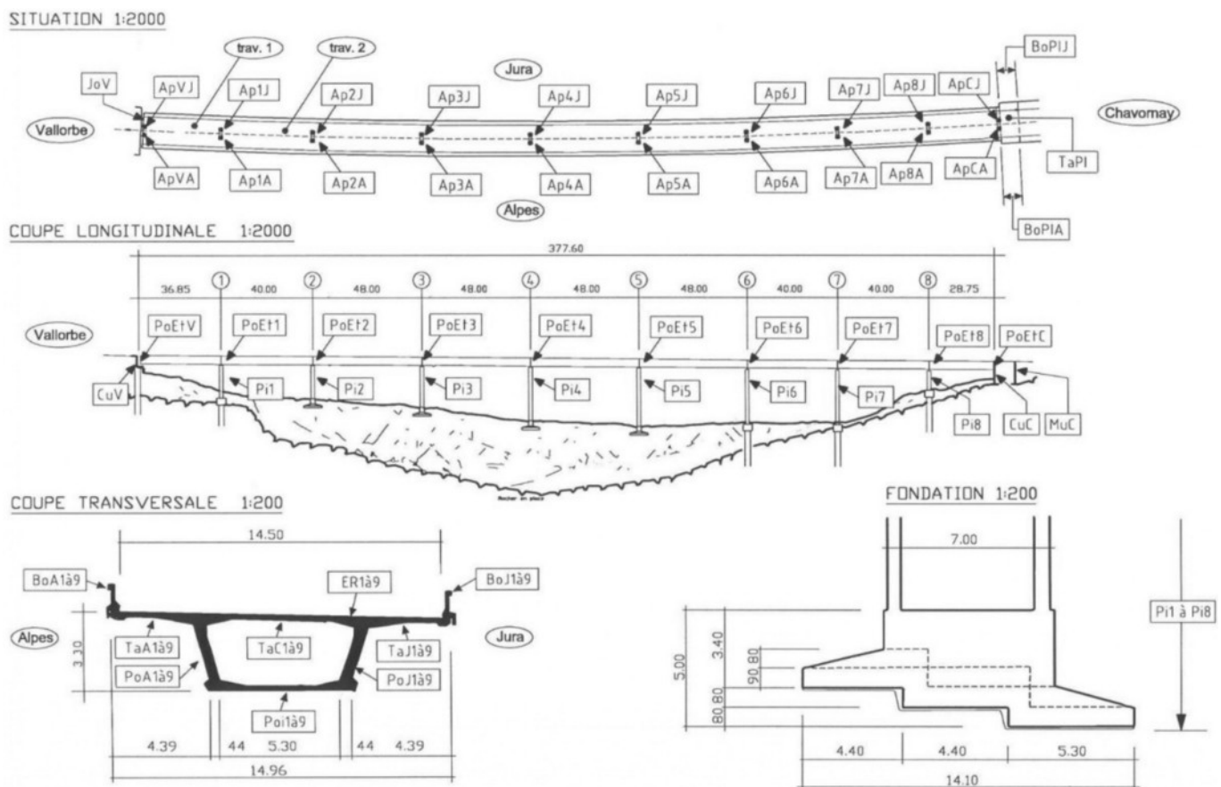
Fig. 4. Comprehensive illustration of bridge Praz: plan, elevation, cross-section, and foundation details.
