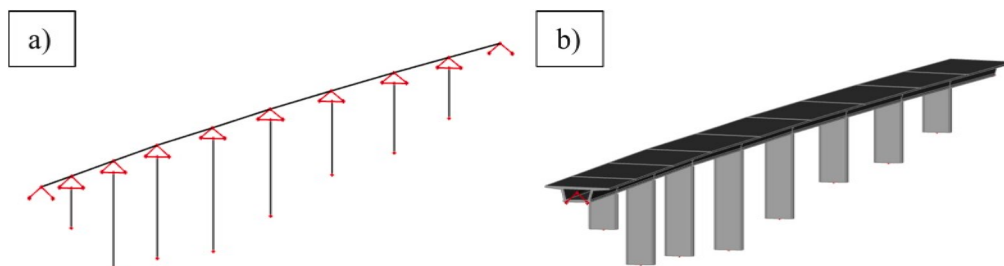
Fig. 12. FE model (Praz Bridge): a) single-line view, b) solid view.
