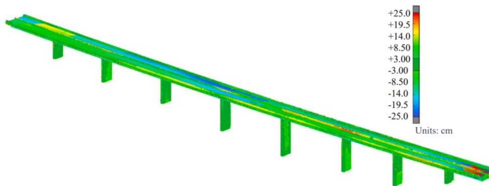
Fig. 9. Deviation between the BIM model and the point cloud (Image courtesy of B. Domer, HEPIA).
