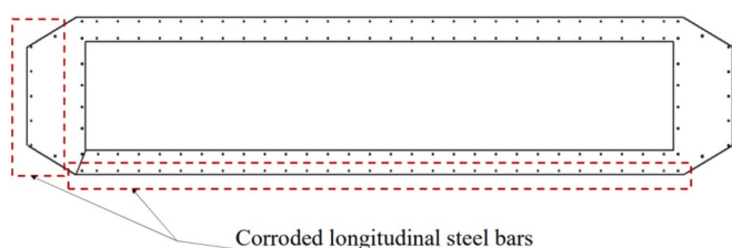
Fig. 14. Disposition of the corroded longitudinal steel bars.
