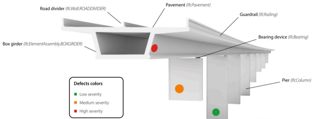
Fig. 10. Degradation visualization model of the Praz bridge [38] (Image courtesy of B. Domer, HEPIA).
