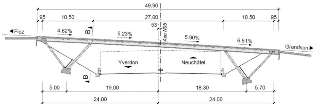
Fig. 16. Longitudinal section of the Grandson bridge.
