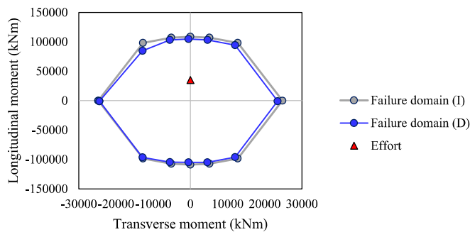
Fig. 13. Bending investigation for pile 5 at the normal stress value of 23,717 kN.
