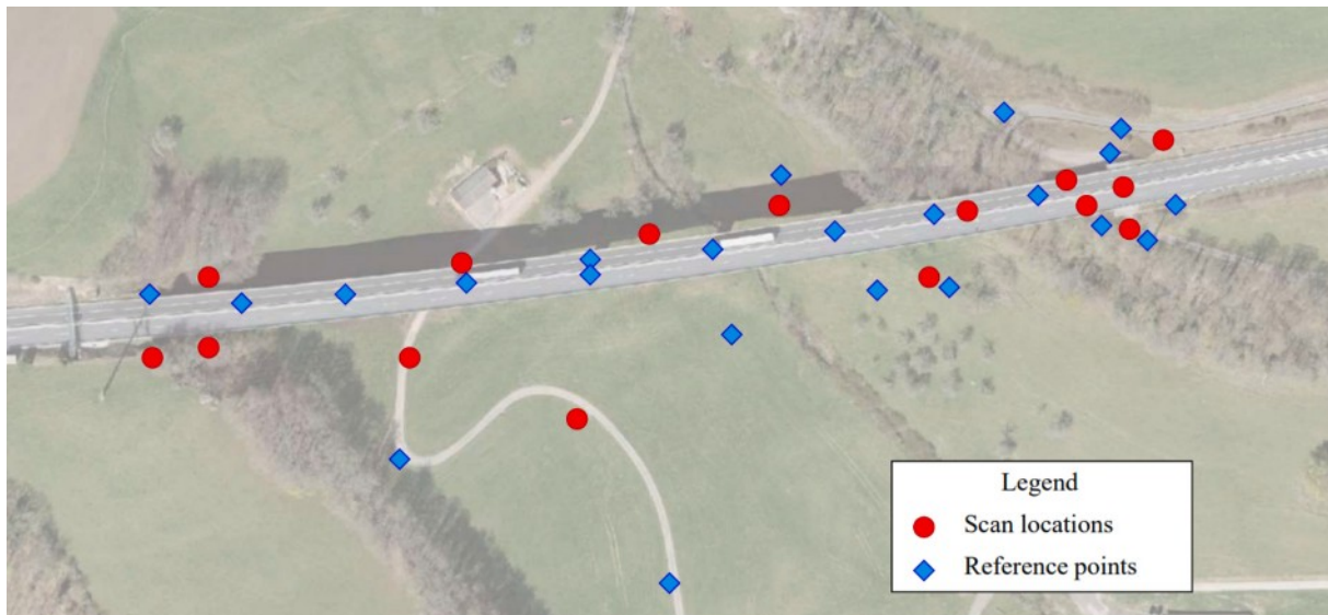
Fig. 5. Locations of scans and reference points on the Praz bridge.
