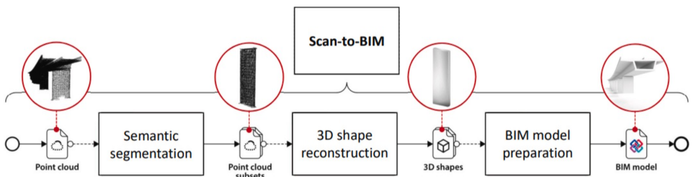
Fig. 7. Scan-to-BIM process overview for creating an IFC 4.3 compatible numerical model (Image courtesy of B. Domer, HEPIA).
