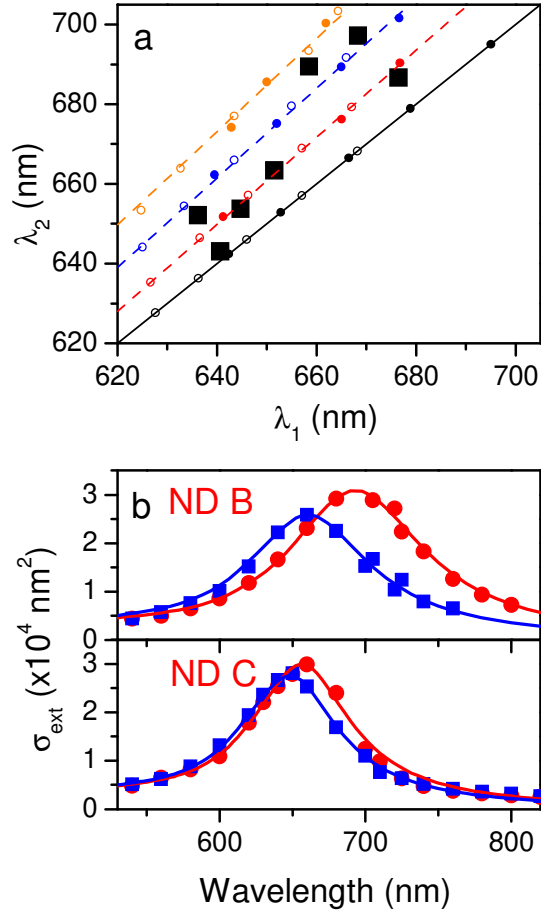
Figure 3. Plasmonic properties of individual gold NDs lithographed on a sapphire substrate. a) Experimental SPR positions \lambda_1 and \lambda_2 of seven individual NDs of same nominal dimensions D=70 nm and h=20 nm (black squares, the symbol size corresponding to experimental uncertainties), measured using SMS for the two orthogonal incident light polarizations yielding maximal and minimal extinction at 700 nm wavelength. Also shown are the computed SPR positions using optical FEM simulations on h=20 nm (full circles) and h=25 nm (hollow circles) NDs with circular or elliptical section of different D_1 and D_2 values, such that D_2/D_1=1 (black circles, corresponding to the case of circular disk with degenerate SPRs, i.e. \lambda_1=\lambda_2 ), 1.05 (red circles), 1.1 (blue circles) and 1.15 (orange circles). Lines correspond to linear fits of the simulated results. b) Extinction spectra of two individual gold NDs (top: ND B, bottom: ND C), measured for two orthogonal light polarizations yielding maximal (red circles) and minimal (blue squares) extinction at 700 nm wavelength, and FEM-simulated spectra (red and blue lines) obtained using morphological parameters yielding an optimal reproduction of the quantitative experimental spectra: h=21.3 nm, D_1=79.9 nm and D_2/D_1=1.14 (ND B) and h=23.7 nm, D_1=78.3 nm and D_2/D_1=1.04 (ND C).
