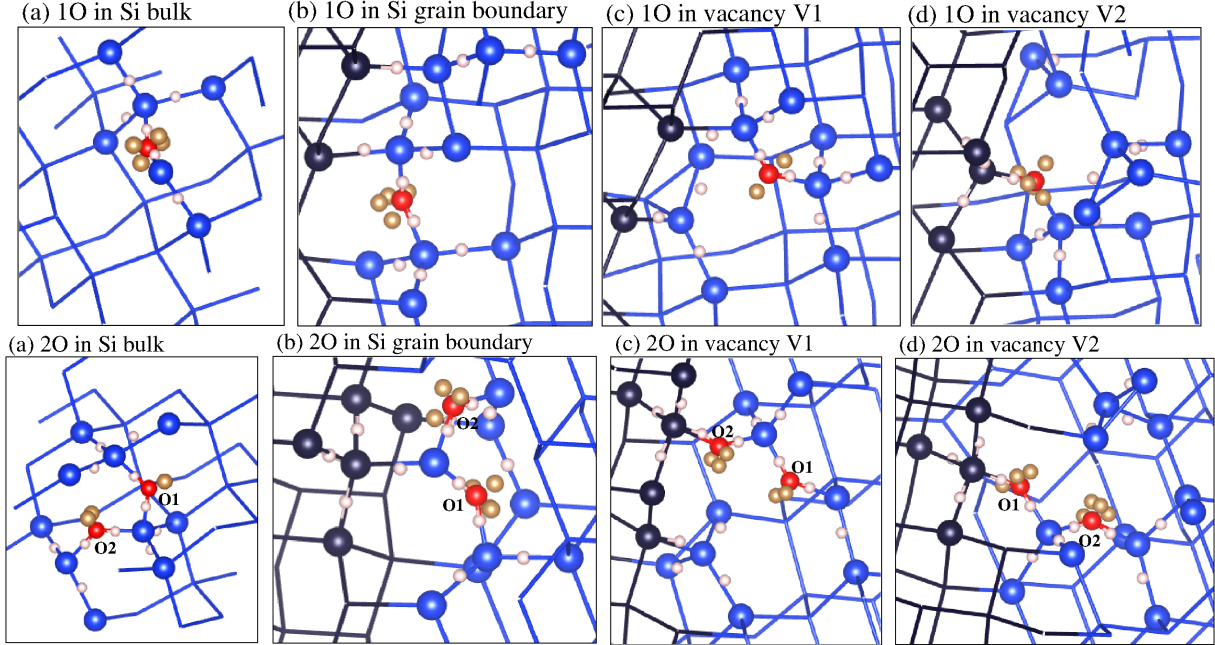
Figure 13. Structures with the inclusion of one oxygen atom (top) and two oxygen atoms (bottom) in a) bulk Si b) GB c) V1 d) V2. Silicon atoms in blue. Bonds and lone pairs are highlighted with small white spheres and brown spheres respectively
