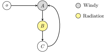
Fig. 1: The Curiosity begins at the origin, o , and then visits the waypoints A , B and C in whichever order is safe. We indicate waypoints with high levels of wind (grey) and radiation (yellow).
