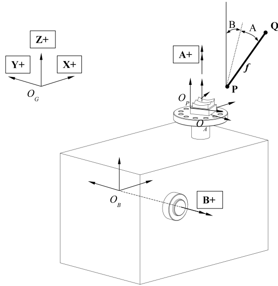
Fig.2 – Machine architecture.
