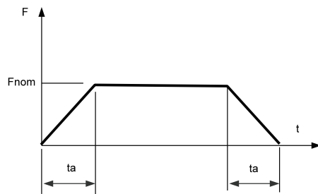
Fig.3 – Motion law
