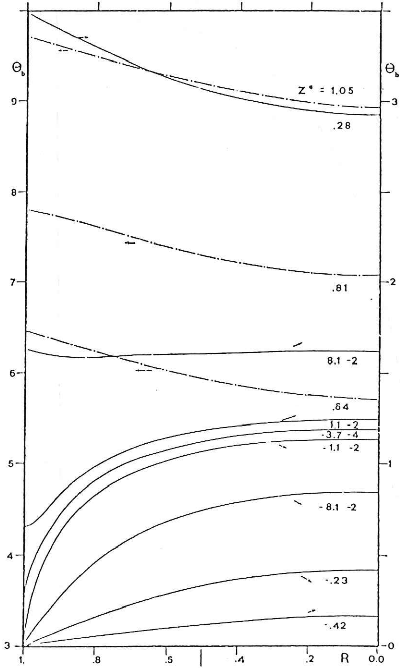
Fig.4 - Temperature distribution for Pe=1 .
