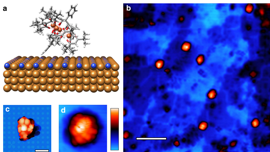
Figure 1 | \text{Fe}_4 molecule adsorbed on the \text{Cu}_2\text{N} surface. (a) [\text{Fe}_4(\text{L})_2(\text{dpm})_6] resting on the \text{Cu}_2\text{N} surface. Adsorption geometry and molecular structure are computed by density function theory (DFT). The molecule's axis defined by the tripodal ligands is at a 33^\circ angle from the surface normal. Atoms are Fe (orange), O (red), C (grey), H (white), Cu (brown) and N (blue). (b) Overview scanning tunnelling microscope (STM) image of the \text{Cu}_2\text{N} surface after deposition of molecules (scale bar, 8 nm). A number of \text{Fe}_4 molecules are visible as the tallest objects in orange. This image was filtered to remove noise using WSxM software 23 . (c) Calculated top view image of relaxed \text{Fe}_4 on \text{Cu}_2\text{N} showing the spatial distribution of the density of states integrated between 0 and +3 eV in energy. (d) STM image of an \text{Fe}_4 molecule. It appears as a spheroid of \sim 2 nm diameter with a multi-lobed substructure consistent with the calculated image in (c). The colour scale indicates the topographical height ranging between 0 and 1 nm in (b,d), which were acquired at a tunnel current set-point of 3 pA and bias voltage of 2.3 V. The 1-nm lateral scale bar inset in (c) also applies to (d).
