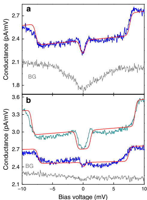
Figure 2 | Conductance spectra of individual molecules. (a) dI/dV(V) spectrum recorded on a molecule with 700 pm topographic height at 0 T magnetic field (blue line, initial current I_0 = 75 pA at V_0 = 10 mV). A background (BG) spectrum recorded with the same tip on bare Cu 2 N is shown in grey. (b) Spectra acquired on a single molecule (800 pm height) without magnetic field (blue line, I_0 = 25 pA, V_0 = 10 mV) and under a 9 T out-of-plane field (green line, I_0 = 50 pA, V_0 = 15 mV), background spectrum (BG, grey line). When a magnetic field is applied, the low-energy excitation widens from 0.2 \pm 0.2 to 0.8 \pm 0.1 mV and the high-energy excitation widens from 7.5 \pm 0.1 to 8.5 \pm 0.1 mV. Background spectra in (a) and (b) are offset for clarity. Red lines in (a) and (b) indicate spectra computed using the spin Hamiltonian model. The fits yield exchange coupling, J = 2.93 meV ( 23.6 cm -1 ), and magnetic anisotropy, D = -52 \mu eV ( -0.42 cm -1 ) for the molecule in (a) and J = 2.89 meV ( 23.3 cm -1 ), D = -26 \mu eV ( -0.21 cm -1 ) with a g factor of 2 for the molecule in (b).
