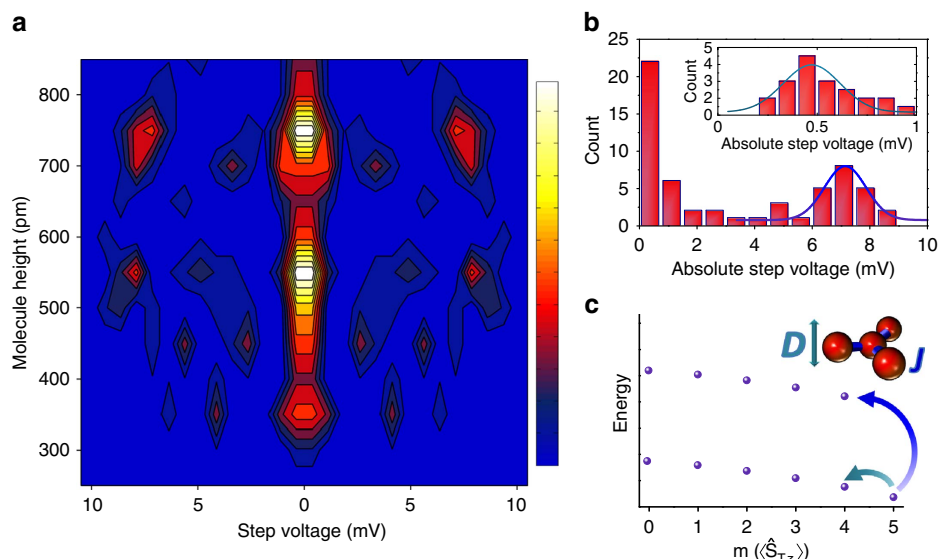
Figure 3 | Spin excitation fingerprint of Fe 4 on Cu 2 N. (a) Two-dimensional histogram for an ensemble of molecules (> 60) correlating zero-field spin excitation energies of a molecule with its topographic height. The histogram counts the number of inelastic tunnelling steps observed in dI/dV(V) binned by step voltage and topographic height of the molecule measured after completion of each spectrum. For molecules over 700 pm in height, a dominant spectrum can be identified. For shorter objects large variation indicates significant changes in magnetic structure and possible fragmentation. Bin sizes are 0.75 mV and 50 pm. The colour scale indicates bin count between 1 and 11. Since spin excitations are symmetric with respect to 0 V, the absolute value of the steps is used, and the symmetrized plot is shown. (b) Histogram of all steps measured on molecules > 700 pm in height. Focusing on those molecules reveals the characteristic spectrum for intact Fe 4 molecules, which features two spin excitations: a low-energy excitation at 0.47 mV and a high-energy excitation at 7.2 mV. Both have broad distributions with standard deviations of 0.14 and 0.7 mV, respectively reflecting variations in spin excitation energies for different molecules. (c) Spin state distribution for Fe 4 single-molecule magnets. States are calculated using a model of the magnetic core (inset) incorporating antiferromagnetic exchange coupling of the three outer Fe ions to the central ion (orange balls) with strength J (blue bonds) and easy-axis magnetic anisotropy with strength D applied to the whole molecule (teal arrow). The characteristic excitations found in (b) are consistent with the two lowest energy transitions excitable by inelastic electron tunnelling (curved teal and blue arrows) with J between 2.5 meV (20 cm -1 ) and 3.1 meV (25 cm -1 ), and D between -34 \mu eV (-0.28 cm -1 ) and -86 \mu eV (-0.70 cm -1 ).
