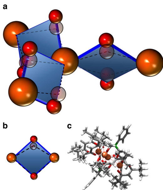
Figure 4 | Structural distortions of Fe 4 in the STM tunnel junction. The strong contact made by the tip induces distortions as the molecule is compressed in the STM junction and enhances super-exchange.
