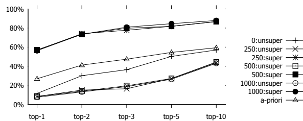
Figure 11: Cumulative accuracy of the forward analysis step applied to the DBLP database without full text indexes.
