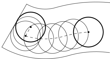
FIGURE 3. The ball-to-ball property of a strip.
