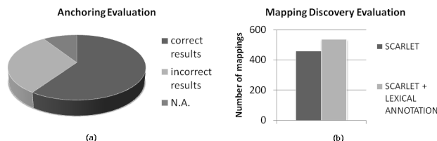
Fig. 5. Lexical annotation evaluation on OAEI 2006 benchmark: detection of incorrect anchoring (a) and new mapping discovery (b)
