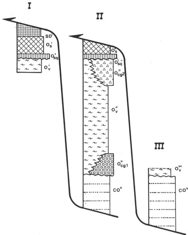
Fig. 4 - Stratigraphic columns and tectonic relation of the three tectonic sub-units within the Hercynian Arburese Tectonic Unit. I) Donigala sub-unit, II) S. Antonio di Santadi sub-unit and III) M. Fonnesu sub-unit.
