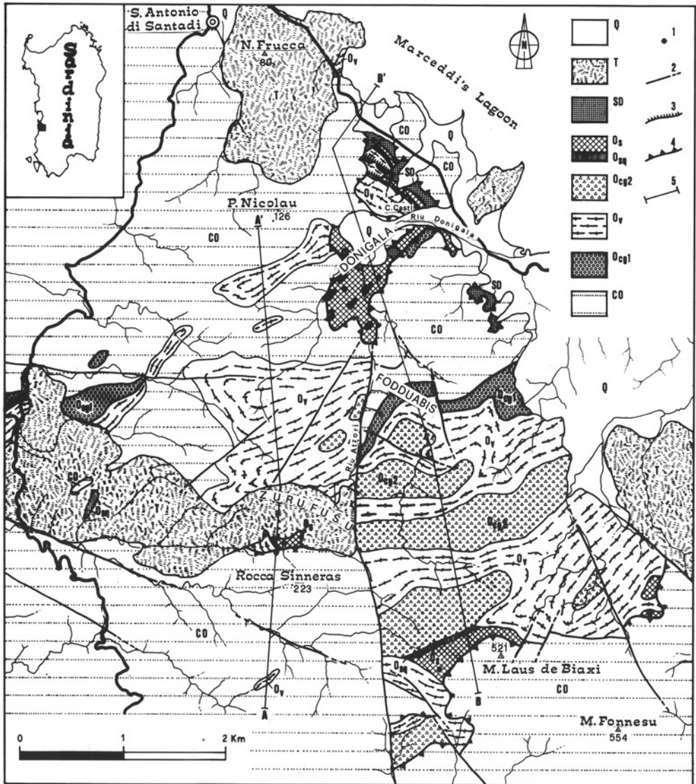
Fig. 1 - Geological sketch-map of the S. Antonio di Santadi area. CO) Cambrian-Lower Ordovician sandstones, siltstones and mudstones. Ocg1) Ordovician (pre-Caradoc) feldspatic sandstones with silty intercalations and conglomerates. Ov) Ordovician (pre-Caradoc) acid volcanites and volcanoclastites. Ocg2) Ordovician (pre-Caradoc) coarse clastic sediments. Osq) Upper Ordovician (Caradoc-Ashgill) coarse and mainly quartzitic detritic sediments. Os) Upper Ordovician (Caradoc-Ashgill) fossiliferous siltstones and sandstones. SD) Silurian-Lower Devonian black fossiliferous limestones and grey nodular limestones. T) Sedimentary and volcanic Tertiary rocks. Q) Quaternary deposits. 1) Fossiliferous outcrops. 2) Faults. 3) Minor overthrusts. 4) Main overthrusts. 5) Location of sections.
