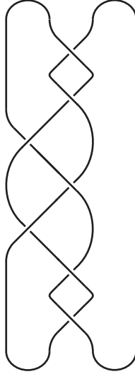
Figure 1: a 4-plat presentation of \mathfrak{b}(21, 8)
