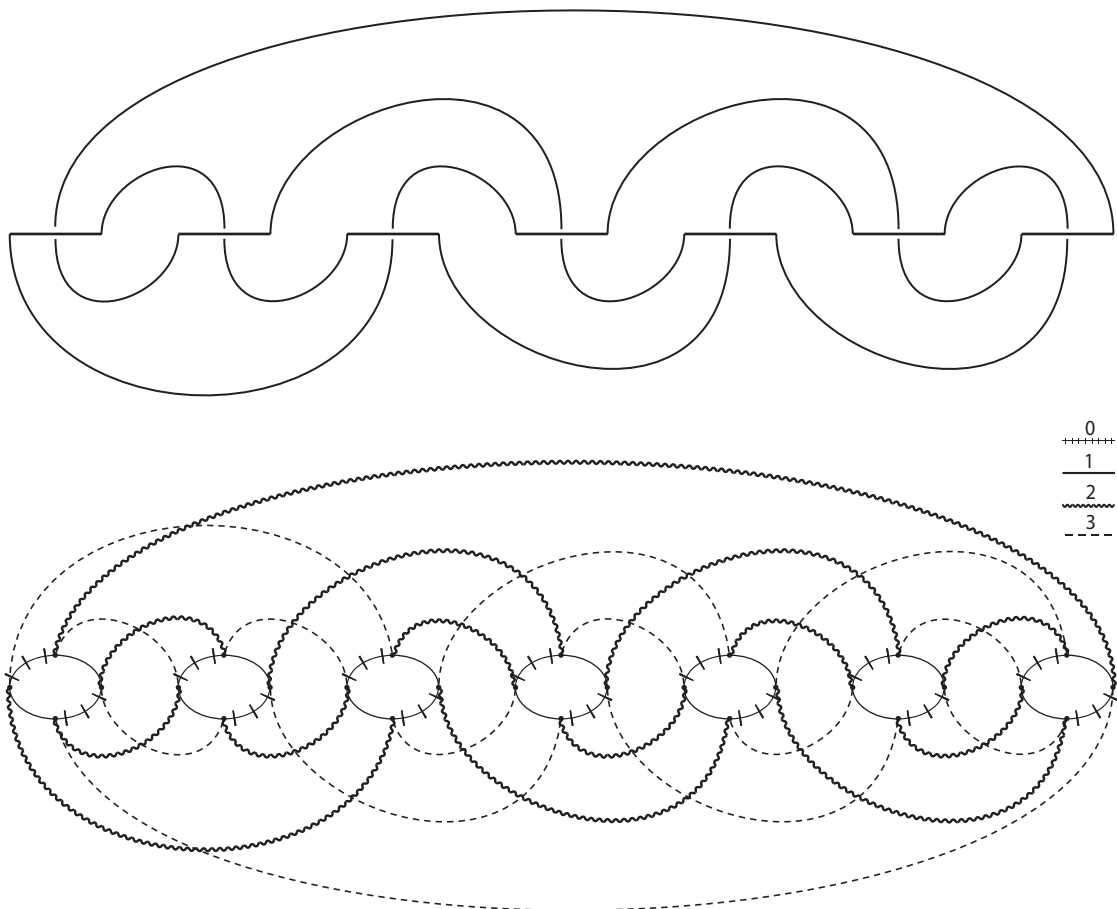
Figure 2: a bridge presentation of \mathfrak{b}(21, 8) and the associated crystallization of L(21, 8)
