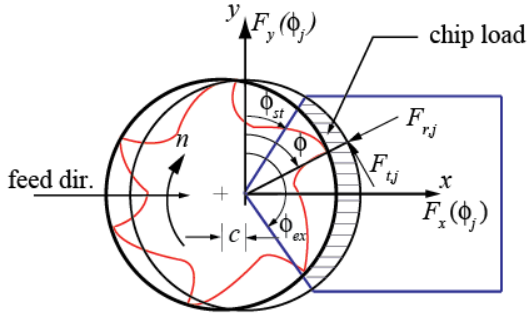
Figure 5. Geometry of milling process [7].
