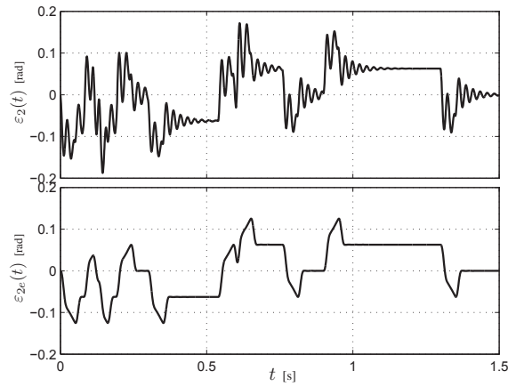
Fig. 22. Comparison between the residual vibration caused by the application to a resonant system G_{ml}(s) of a second order trajectory q_2(k) ( \varepsilon_2(t) ) and the corresponding exponential jerk trajectory q_{2e}(k) shown in Fig. 21 ( \varepsilon_{2e}(t) ).
