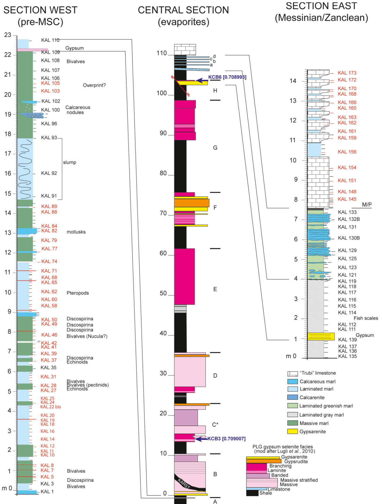
Fig. 3. Kalamaki composite section (west subsection: 37°44o11.95"N, 20°54o13.14"E; east subsection: 37°44o12.62"N, 20°54o19.09"E)
