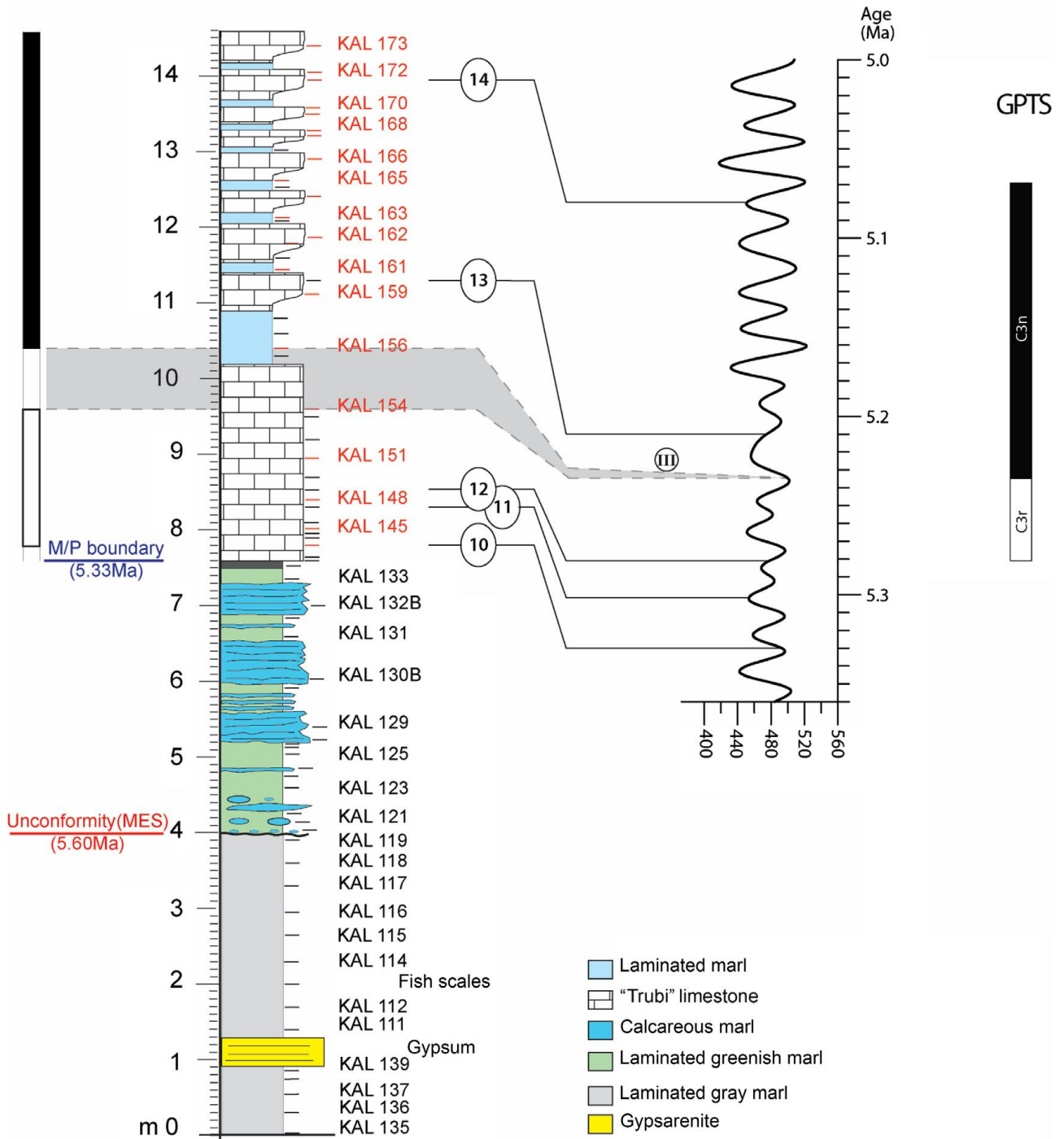
Fig. 16. Kalamaki section age model of the PLG top portion, Lago Mare, and Trubi Formation, correlated with insolation curve (based on Laskar et al., 2004). Bio-magnetotaxonomic events are as follows: 10) N. acostaensis influx sinistral; 11) Sphaeroidinellopsis spp. AB; 12) N. acostaensis influx sinistral; 13) Sphaeroidinellopsis spp. AE; 14) FCO G. margaritae ; III) boundary C3r/C3n. (full data are available as supplementary material).
