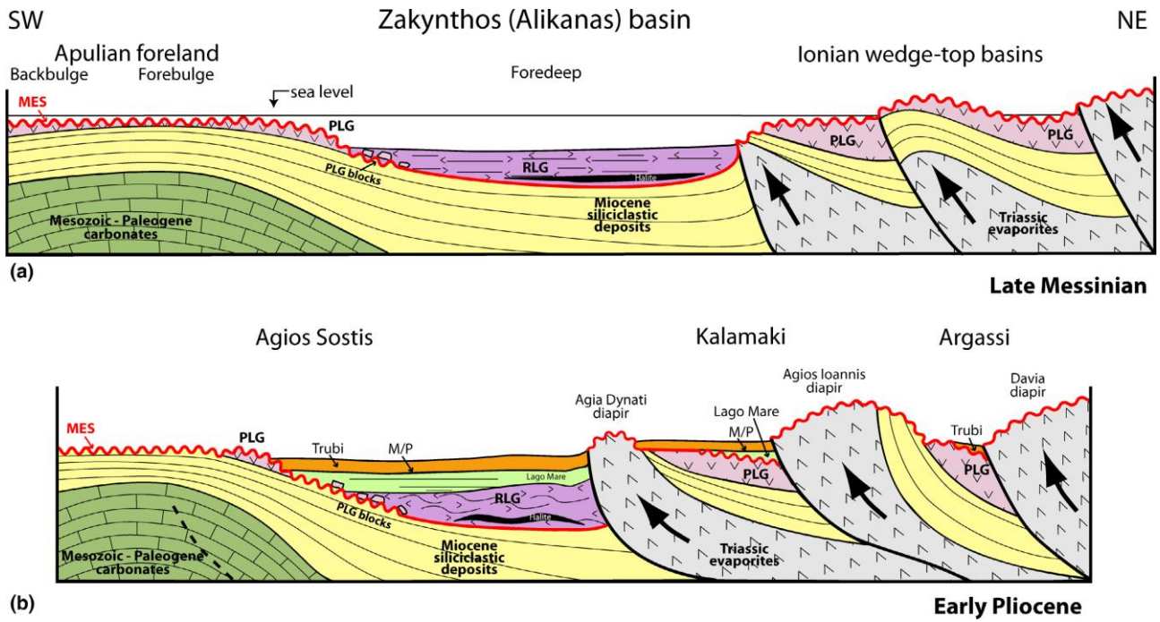
Fig. 17. Palaeogeographic reconstruction. (a) During the Messinian, the Zakyntos (Alikanas) foreland basin was formed in front of the Ionian thrust. The Neogene formations deposited over the pre-Apulian domain corresponded to the foredeep and the flank between foredeep and forebulge, whereas those overlying the Ionian zone corresponded to the wedge-top, which was uplifted due to the diapiric movements of the Ionian Triassic evaporites. In the 1st MSC stage, PLG was deposited on both forebulge and wedge-top. In the 2nd MSC stage, PLG was totally or partially eroded (creating the Messinian Erosional Surface; MES) and redeposited with correlative conformity mainly as gypsum turbidites (RLG unit) in the depocentre of the foreland basin. (b) During the end of the Messinian, in Kalamaki–Argassi wedge-top area the Lago Mare sediments were unconformably overlying the Primary Lower Gypsum above the MES, whereas in the depocentre of the foreland basin they were conformably deposited over the Resedimented Lower Gypsum. The Zanclean flood was recorded on both areas by the conformable deposition of the Trubi Formation. With red raffled and continuous line the unconformity and the correlative conformity of the MES, respectively.
