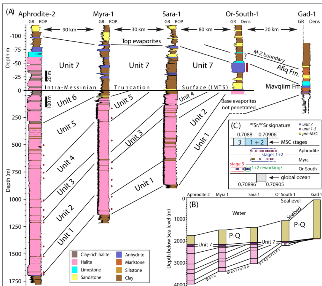
Figure 3. A: Stratigraphic correlation section through Aphrodite-2, Myra-1, Sara-1, Or-South-1, and Gad-1 well (Levant Basin), flattened according to the Intra-Messinian Truncation Surface (IMTS) at the base of Unit 7 (stage 2–3 transition). Note the different vertical scales below and above the IMTS. Lithology in Aphrodite-2, Myra-1, and Sara-1 is based on GR, RES, and ROP (rate of penetration) logs. Lithology in Or-South and Gad-1 is based on wireline logs confirmed by biostratigraphy and sedimentology analyses (Derin, 2000; Hilton, 2001; Buchbinder et al., 2006). The presence of halite within the lower part of Unit 7 in Aphrodite-2 may represent reworking of halite clasts downslope following the initial stage of dissolution. Red circles indicate position of samples for ^{87}\text{Sr}/^{86}\text{Sr} analyses. b) Structural geometry of the MSC section and the Pliocene-Quaternary (P-Q) overburden between studied wells with no flattening and relative to sea-level. C: Results of ^{87}\text{Sr}/^{86}\text{Sr} analyses. Note the clear distinction between stage 1+2 values found in the halite units and stage 3 values found in unit 7 (details about Sr values typical to the three stages of the MSC are presented by Roveri et al. [2014c]). A few intermediate values found in Unit 7 in Or-South probably represent reworked gypsum derived from stage 1 or stage 2 sulfates. Symbols are larger than error bars (2 standard error; min 6 ppm; max 15 ppm; average 9 ppm; further information is provided in the Data Repository [see footnote 1]).
