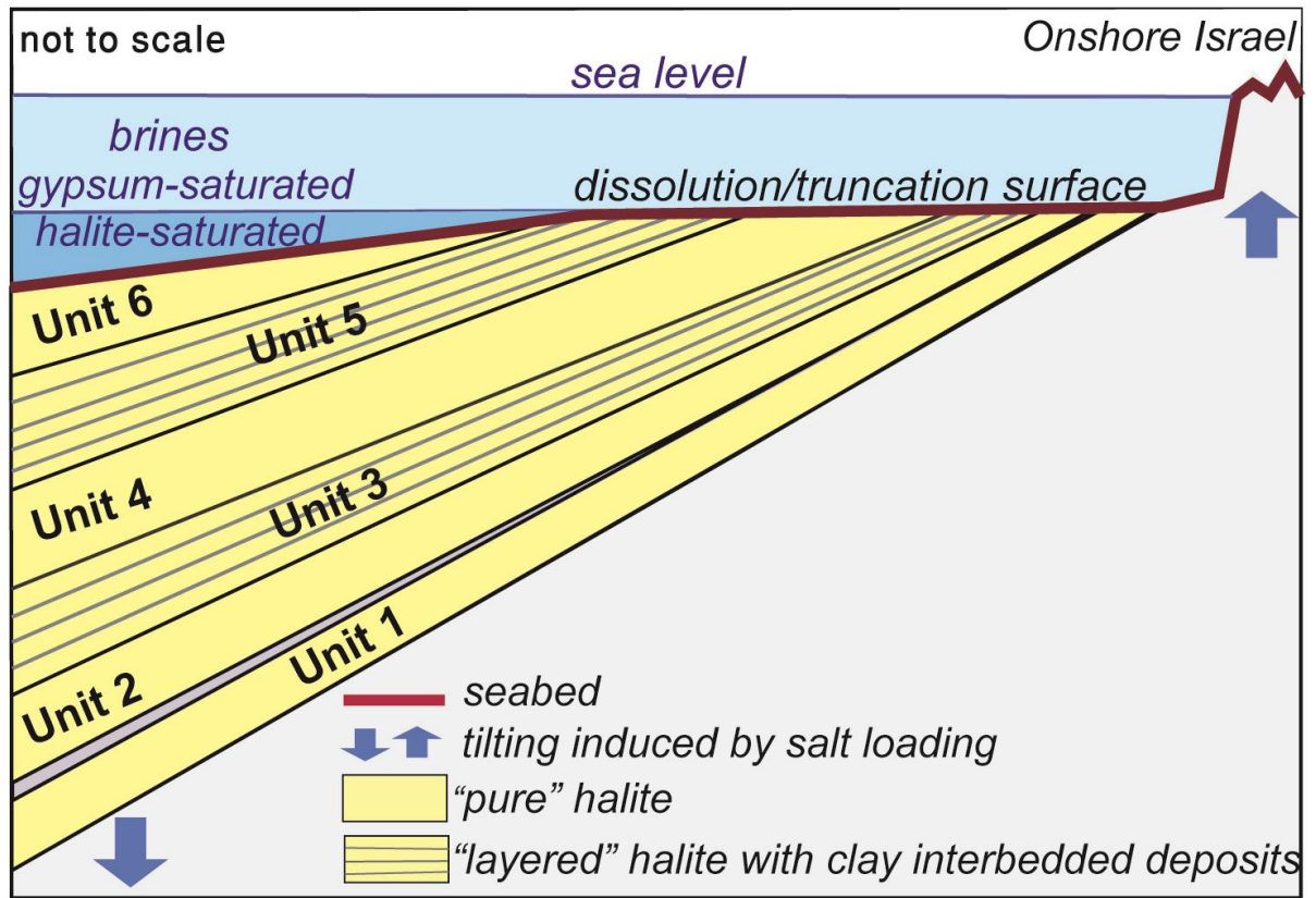
Figure 4. Model for submarine dissolution of a tilted evaporitic sequence above a horizontal chemocline separating a lower halite-saturated hypolimnion from upper under saturated epilimnion.
