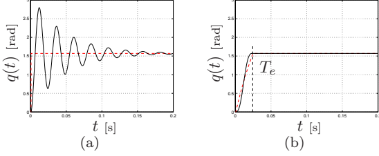
Fig. 5. Response of a lightly damped vibratory system G_{ml}(s) to a step input q_{ref}(t) (a), compared to the response caused by the step filtered by F_e^{\alpha k}(s) (b). Reference trajectories are in red dashed line.
