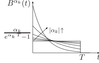
Fig. 1. Exponential basis-function B^{\alpha_k}(t) for different values of parameter \alpha_k < 0 .
