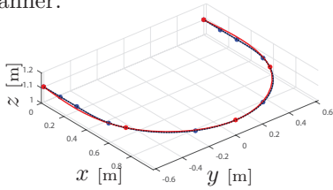
Fig. 9. Desired geometrical path (in black) and approximating B-splines: in blue is the standard B-spline, in red is the exponential tension B-spline. Via-points are reported with circles.
