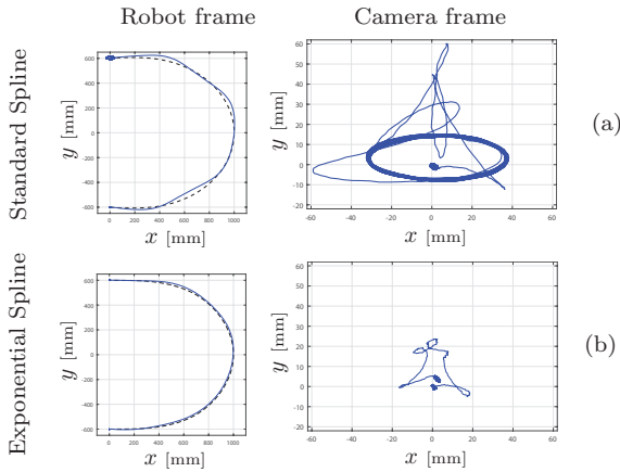
Fig. 11. Pendulum motion when applying the standard B-spline trajectory (a) and the exponential B-spline (b).
