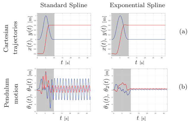
Fig. 10. B-spline trajectories in cartesian coordinates (a) and respective pendulum motion (b).
