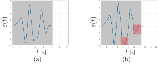
Fig. 6. Responses of a second order system ( \delta = 0.2 , \omega_n = 2\pi ) fed by exponential tension B-splines: in (a) nominal parameter are used while in (b) \omega_n is assumed 30% lower than the nominal value. In red vibrations occurring during the motion are highlighted.
