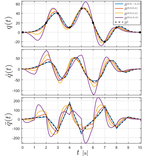
Fig. 4. Position, velocity and acceleration profiles of (scalar) uniform B-spline trajectories using the different basis functions of Fig. 3 with T = 1 and \hat{\alpha} = -1.7 .
