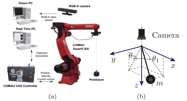
Fig. 8. Experimental setup based on an industrial manipulator (a) and pendulum motion description in terms of angles \theta_1 and \theta_2 (b).
