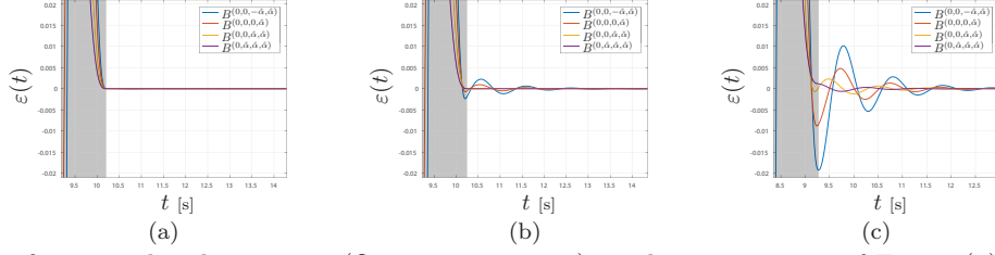
Fig. 7. Responses of a second order system ( \delta = 0.2 , \omega_n = 2\pi ) to the trajectories of Fig. 4 (a) and responses of the same system assuming the presence of a 10% error in the estimation of parameter \delta (b) and \omega_n (c).
