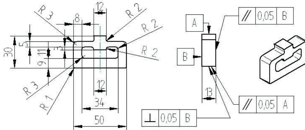
Fig. 1: Geometry and dimensions of the specimen.
