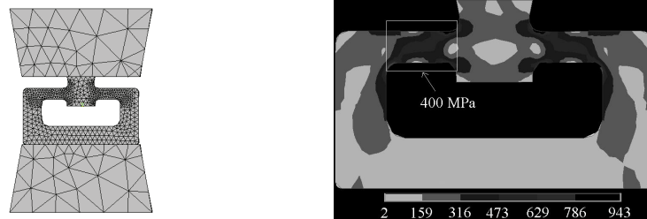
Fig. 2 (left) FE model of the tool-specimen contact and (right) Von Mises stress distribution in the specimen (400 MPa being the average value of the stress in the bridge of the specimen).
