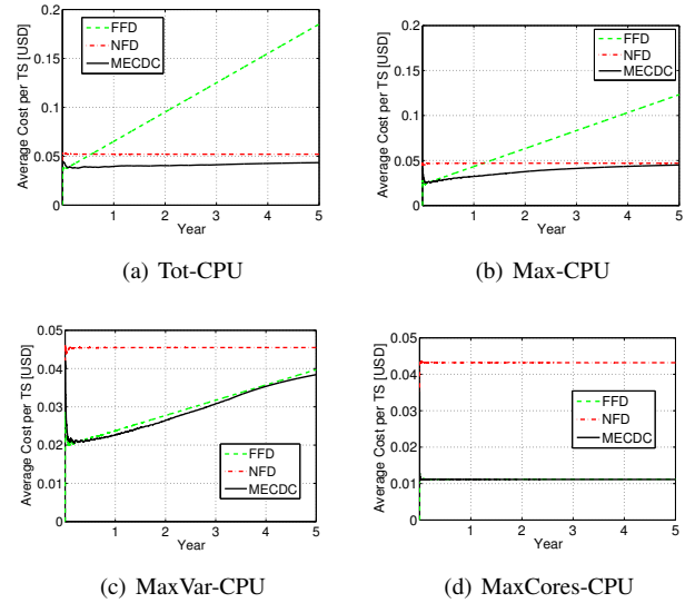
Fig. 6. Average cost per TS vs. time across the different VMs subsets considering MECDC, FFD, NFD.
