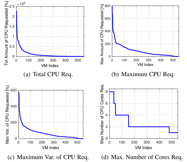
Fig. 3. VMs ordered according to different rules (Note: the VM indexes change between one ordering rule and another one).
