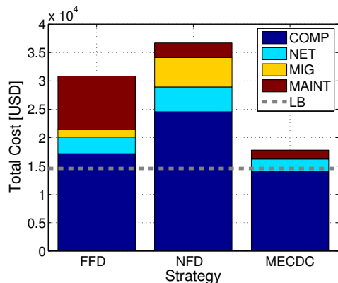
Fig. 7. Costs breakdown at the end of the considered 5-years period for the Tot-CPU subset and the heterogeneous PSs set considering MECDC, FFD, NFD and the Lower Bound (LB).
