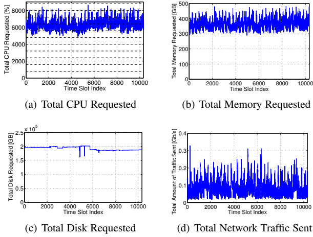
Fig. 2. Evolution of the CPU, memory, disk and network traffic vs TS index for the considered DC trace.
