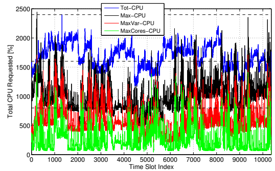
Fig. 4. Total Variation of CPU vs. the TS index for the different VM subsets.
