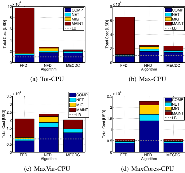
Fig. 5. Costs breakdown at the end of the considered 5-years periods across the different VMs subsets considering MECDC, FFD, NFD and the Lower Bound (LB).
