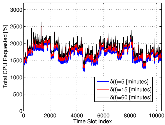
Fig. 8. Total Variation of CPU vs. the TS index for different TS duration \delta(t) (Tot-CPU subset).
