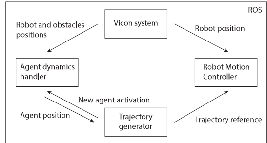
Fig. 10. Overall conceptual scheme of the trajectory planner in ROS.
