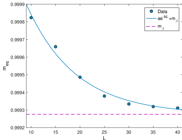
FIG. 6. Time-averaged magnetization on the last column m_{eq} at equilibrium (i.e. without reservoirs) versus system size L . The horizontal line is m_{\beta} \approx 0.99927 . The continuous line is an exponential fit m_{\beta} + ae^{-bL} with a = 0.0015 \pm 0.0004 and b = 0.10 \pm 0.02 .
