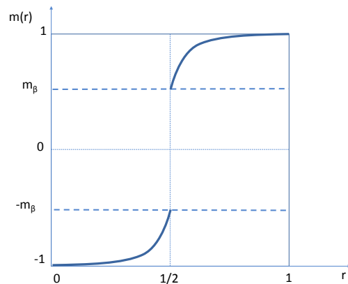
FIG. 3. Sketch of the magnetization profile m(r) in the macroscopic coordinate r = x/L ( r \in [0, 1] ), when m_+ = 1 .
