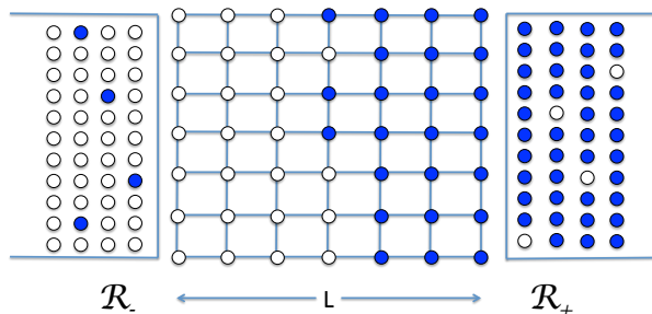
FIG. 1. Schematic picture of the 2D Ising model coupled to reservoirs \mathcal{R}_+ and \mathcal{R}_- . A spin up is represented with a filled (blue) circle, a spin down is represented with an empty (white) circle.
