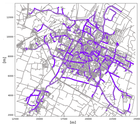
Figure 4: Simulated area with roads that have a significant number of vehicles (above 1000 veh/day) colored in purple.
