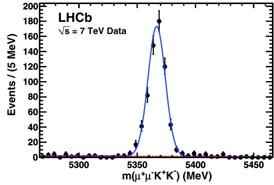
Fig. 3. The invariant mass of J/\psi K^+K^- combinations when the K^+K^- pair is required to be within \pm 20 MeV of the \phi mass. The data have been fit with a Gaussian signal function whose mass and width are allowed to float and linear background function shown as a dashed line. The solid curve shows the sum.
