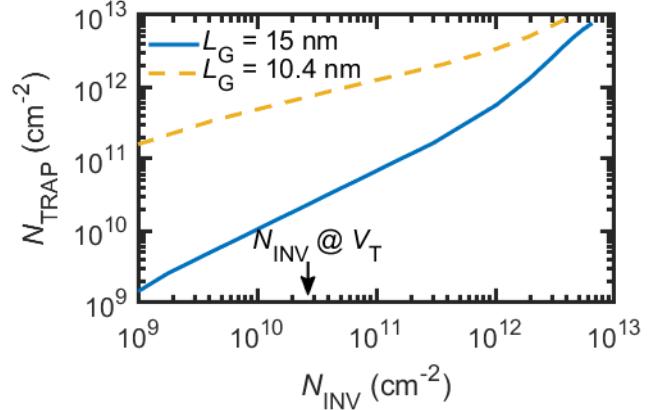
Fig. 6. N_{\text{TRAP}} vs N_{\text{INV}} for the 15-nm (blue solid curve) and 10.4-nm (yellow dashed curve) devices. The channel thickness t_{\text{CHAN}} is 7 nm and 4 nm, respectively. The N_{\text{INV}} for the results in Fig. 5, i.e. at threshold condition, is indicated. The increase in trapped charge density for lower t_{\text{CHAN}} is explained by the deeper penetration of the Fermi-level in the conduction band, thus probing the trap distribution where the trap density is higher, see Fig. 2a).
