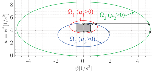
Fig. 4: Plane \check{\psi} - \psi^2 with the three ellipses \Omega_i , rectangle R_\psi (in gray) and curve \Gamma_\psi (black line). Notice how R_\psi \in \Omega_1 \cap \Omega_2 \cap \Omega_3 and \Gamma_\psi \in R_\psi .
