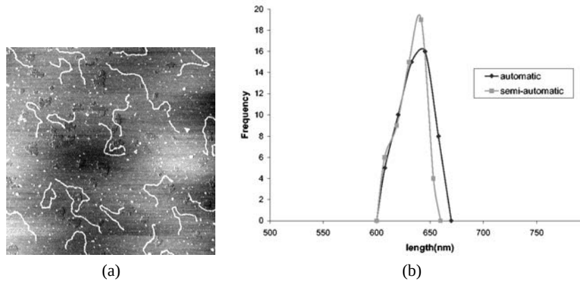
Fig. 9. (a): PstI-PstI dimer DNA molecules in an AFM image; (b): Histogram of PstI-PstI dimer molecules sizing: the solid plot represents our measures, the dashed plot represents the semi-automated measures
