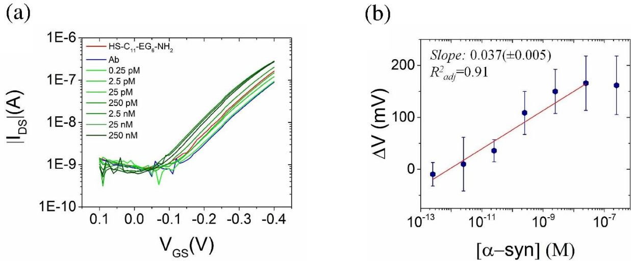
Figure 6. (a) Transfer characteristics ( V_{DS} = -0.1 V) of the sensing experiment employing the EGFET with Ab-SAM-coated coplanar-gate Au gate and (b) relative calibration curve.
