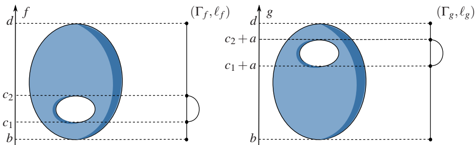
FIGURE 16. The example used in the proof of Corollary 5.9 to show that the edit distance between labeled Reeb graphs can be more discriminative than the functional distortion distance between Reeb graphs whenever the same functions are considered.
