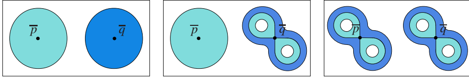
FIGURE 7. Two critical points in different connected components of the same critical level. The dark (resp. light) regions correspond to points below (resp. above) this critical level. Possibly inverting the colors of one or both the components, we have all the possible cases.
