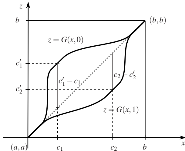
FIGURE 14. The function G introduced in [18] and used in the proof of Lemma 5.5.
