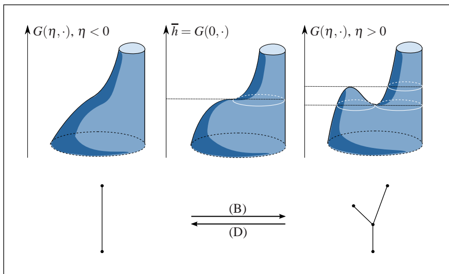
FIGURE 6. Center: A function \bar{h} \in \mathcal{F}_\alpha^1(\mathcal{M}) ; left-right: The universal deformation G(\eta, \cdot) with the associated labeled Reeb graphs for \eta < 0 and \eta > 0 .
