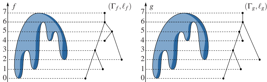
FIGURE 15. The example used in the proof of Corollary 5.8 to show that the edit distance between labeled Reeb graphs can be more discriminative than the bottleneck distance between persistence diagrams whenever the same functions are considered.
