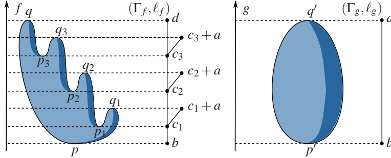
FIGURE 5. The functions f, g \in \mathcal{F}^0(\mathcal{M}) considered in Example 1.
