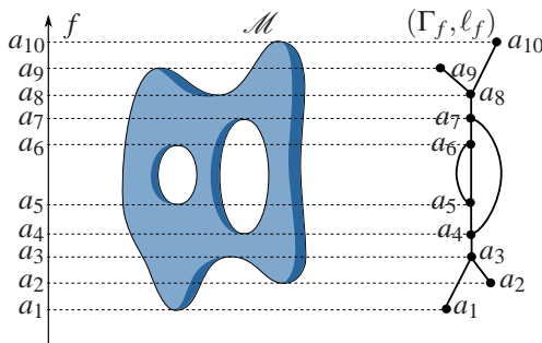
FIGURE 2. Left: the height function f : \mathcal{M} \rightarrow \mathbb{R} ; center: the surface \mathcal{M} of genus g = 2 ; right: the associated labeled Reeb graph (\Gamma_f, \ell_f) .
