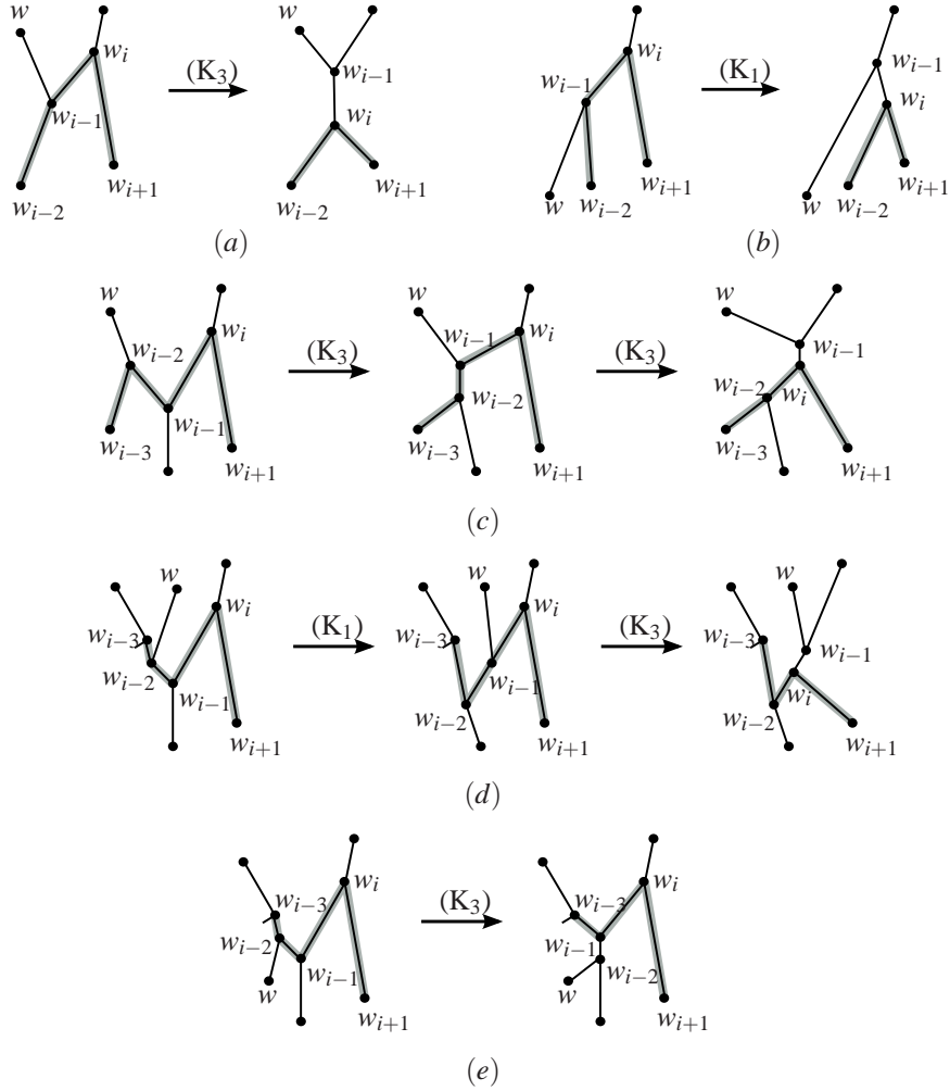
FIGURE 3. Possible configurations of a simple path on a labeled Reeb graph in a neighborhood of its maximum point, and elementary deformations which reduce its length. To facilitate the reader, f has been represented as the height function, so that \ell_f(w_a) < \ell_f(w_b) if and only if w_a is lower than w_b in the pictures.
