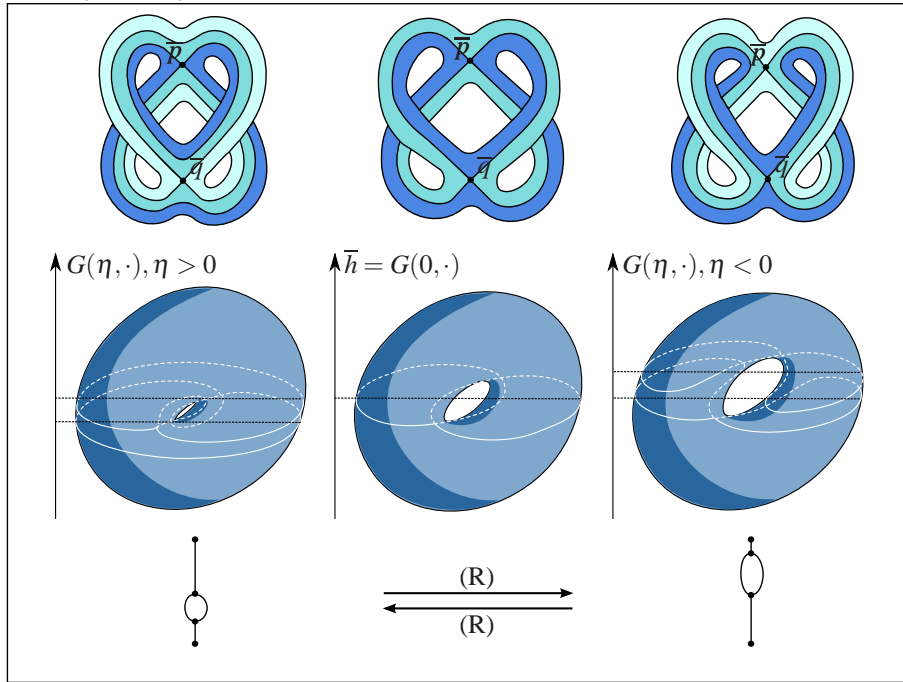
FIGURE 13. Center: A function \bar{h} \in \mathcal{F}_\beta^1(\mathcal{M}) as in case (2) with \bar{p}, \bar{q} as in Figure 8 (d); left-right: The universal deformation G(\eta, \cdot) with the associated labeled Reeb graphs for \eta < 0 and \eta > 0 .
