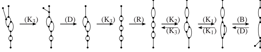
FIGURE 4. Using the procedure followed in the proof of Proposition 2.7, the leftmost labeled Reeb graph is transformed into the rightmost one applying first the deformation which reduces the former into its canonical form, then an elementary deformation of type (R), and eventually the inverse of the deformation which reduces the latter into its canonical form.
