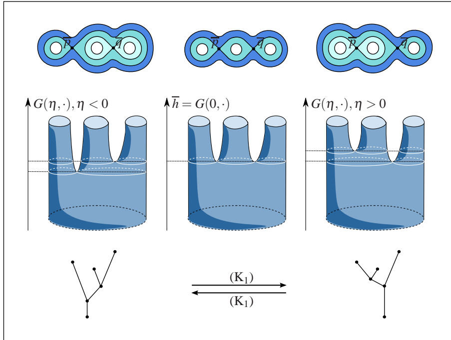
FIGURE 10. Center: A function \bar{h} \in \mathcal{F}_\beta^1(\mathcal{M}) as in case (2) with \bar{p}, \bar{q} as in Figure 8 (a); left-right: The universal deformation G(\eta, \cdot) with the associated labeled Reeb graphs for \eta < 0 and \eta > 0 .
