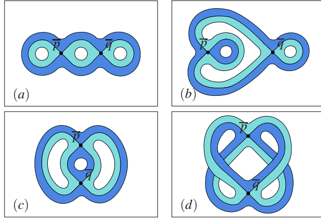
FIGURE 8. Two critical points in the same connected component of the same critical level. The dark (resp. light) regions correspond to points below (resp. above) this critical level. Possibly inverting the colors of this component, we have all the possible cases.
