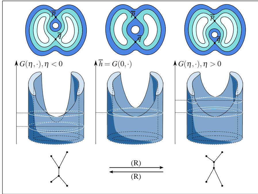
FIGURE 12. Center: A function \bar{h} \in \mathcal{F}_\beta^1(\mathcal{M}) as in case (2) with \bar{p}, \bar{q} as in Figure 8 (c); left-right: The universal deformation G(\eta, \cdot) with the associated labeled Reeb graphs for \eta < 0 and \eta > 0 .
