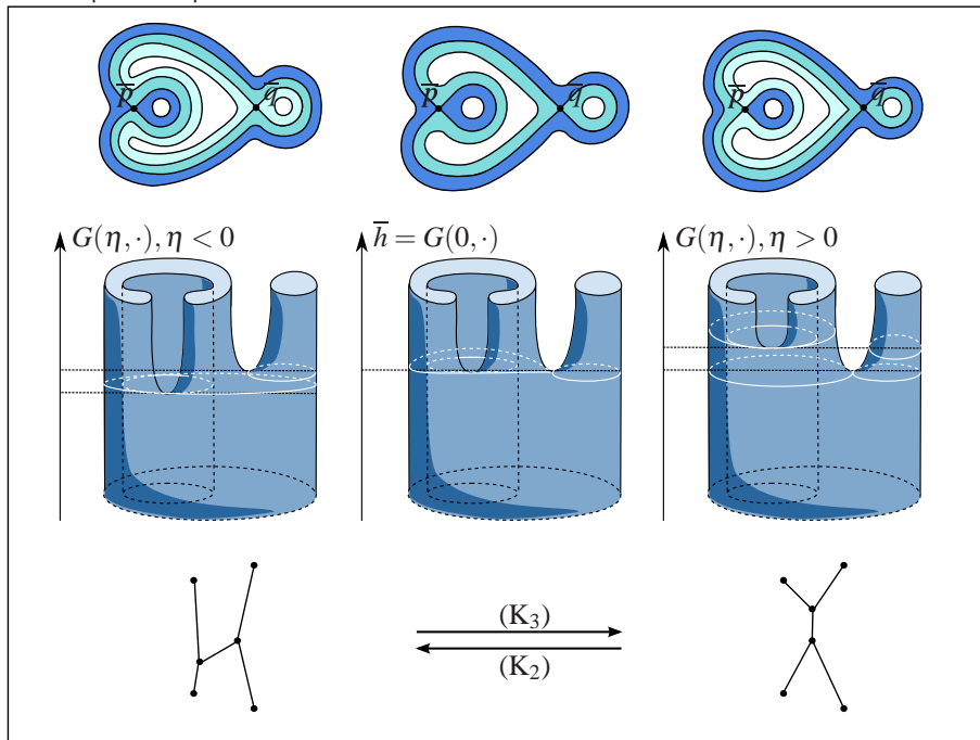
FIGURE 11. Center: A function \bar{h} \in \mathcal{F}_\beta^1(\mathcal{M}) as in case (2) with \bar{p}, \bar{q} as in Figure 8 (b); left-right: The universal deformation G(\eta, \cdot) with the associated labeled Reeb graphs for \eta < 0 and \eta > 0 .
